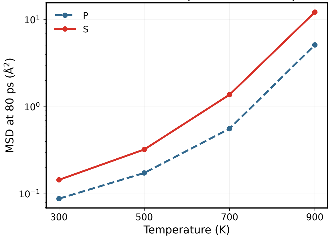
b Host-framework displacement at 80 ps
