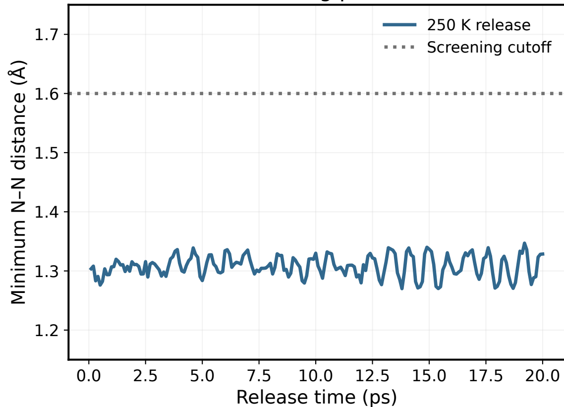
N-N distance during pressure release
