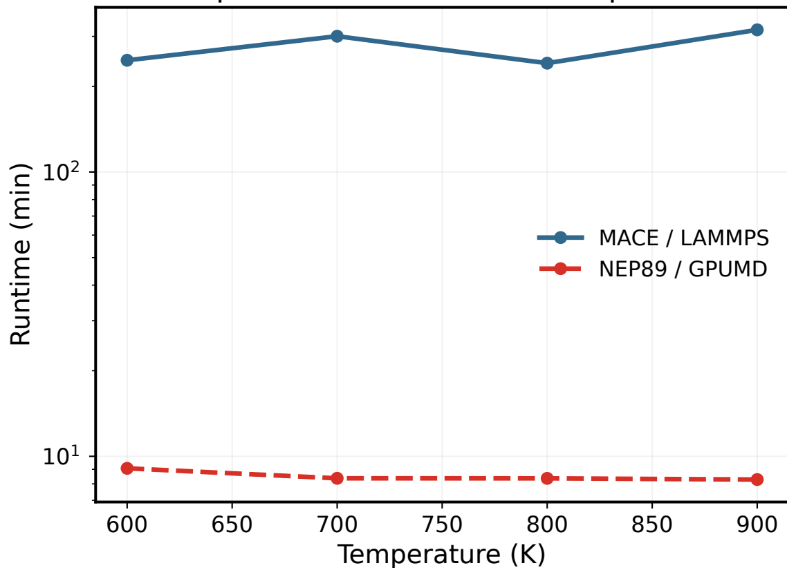
Computational cost across temperature
