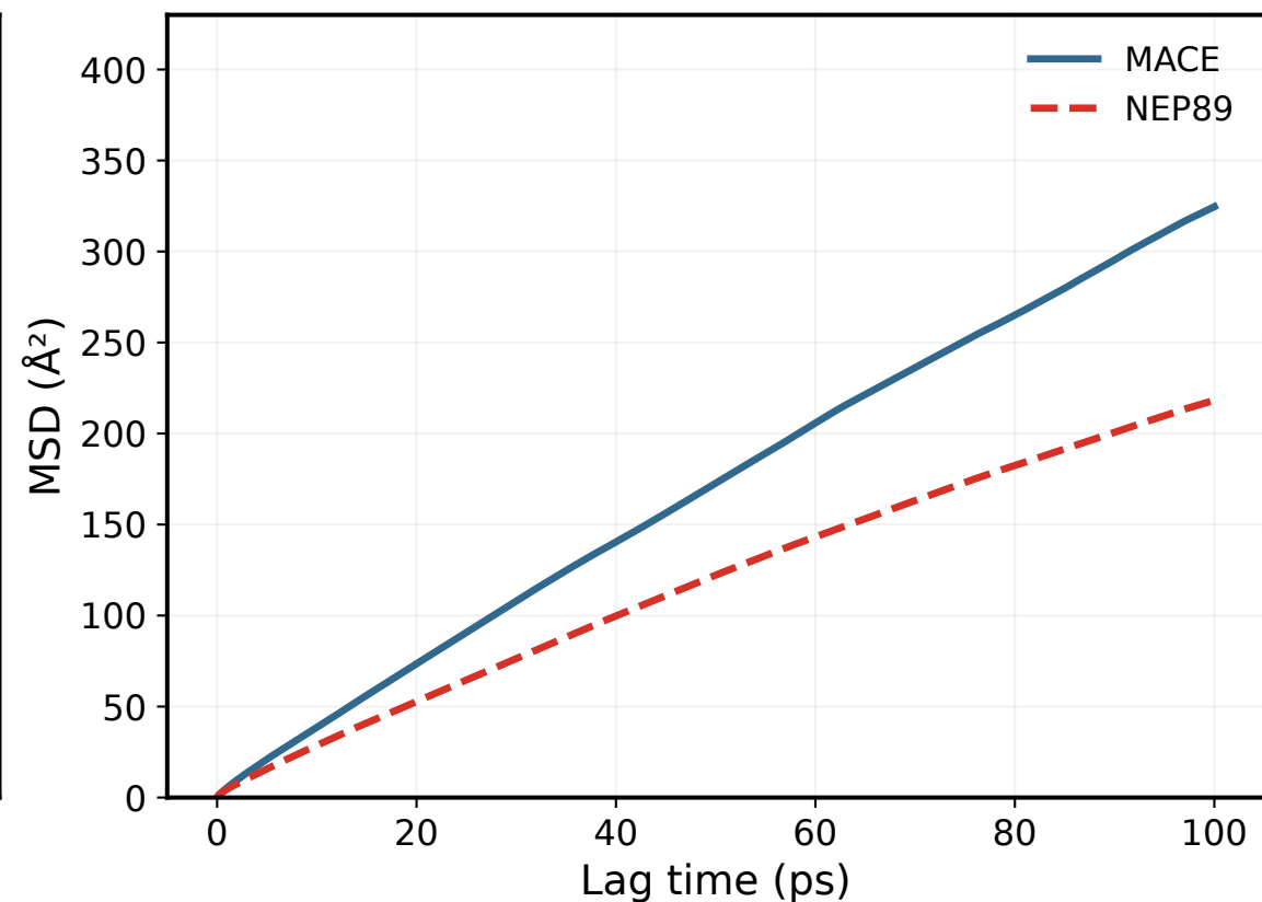
Framework MSD at 900 K
