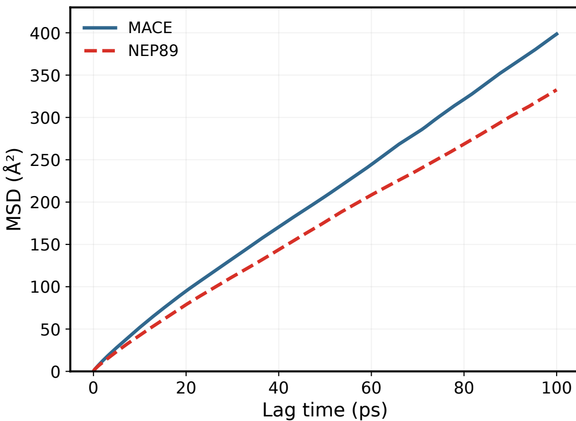
Lithium MSD at 900 K
