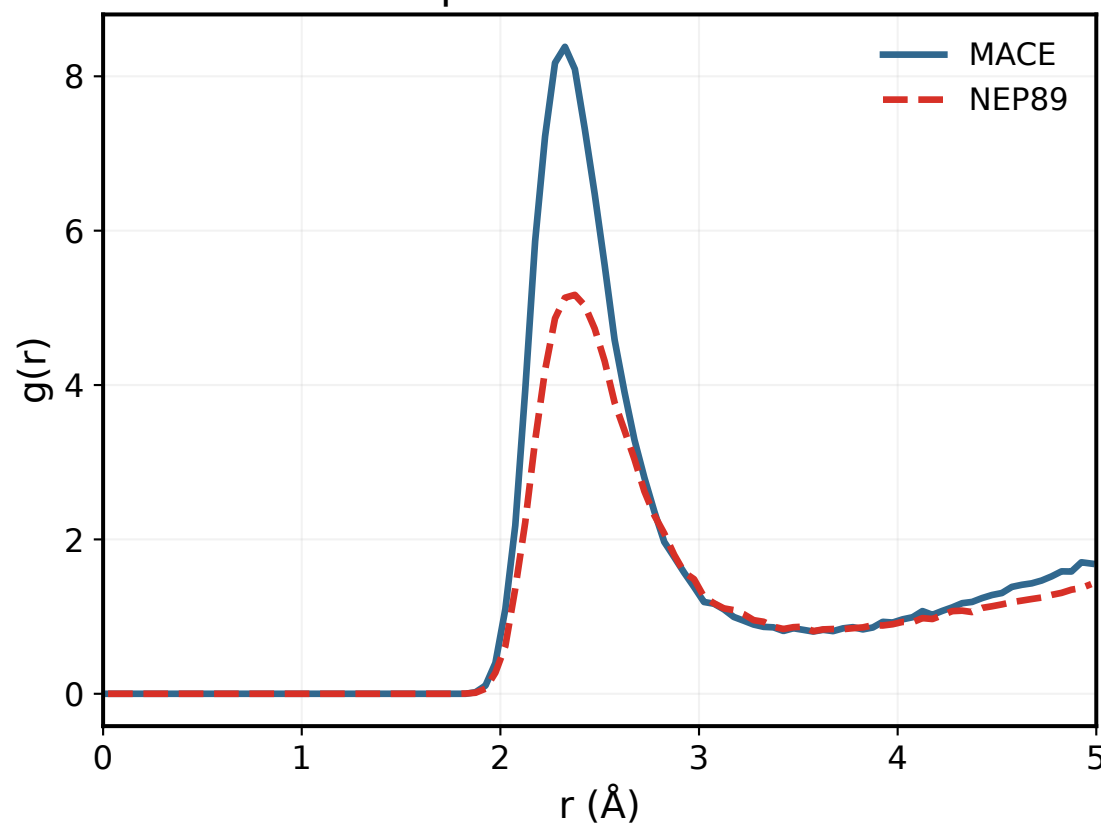
Zr-Cl partial RDF at 900 K
