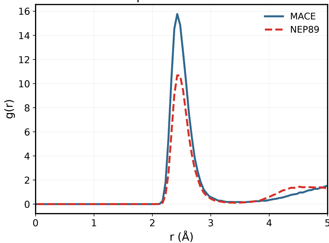
Zr-Cl partial RDF at 900 K
