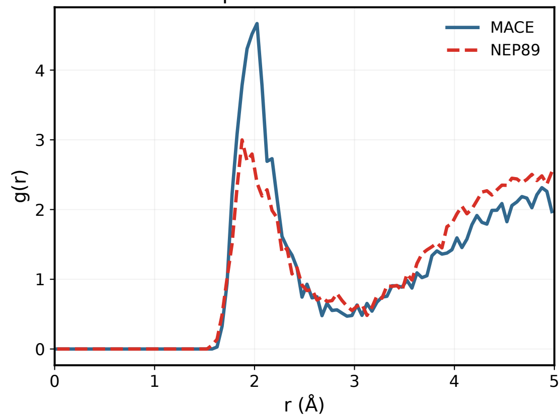
Zr-O partial RDF at 900 K
