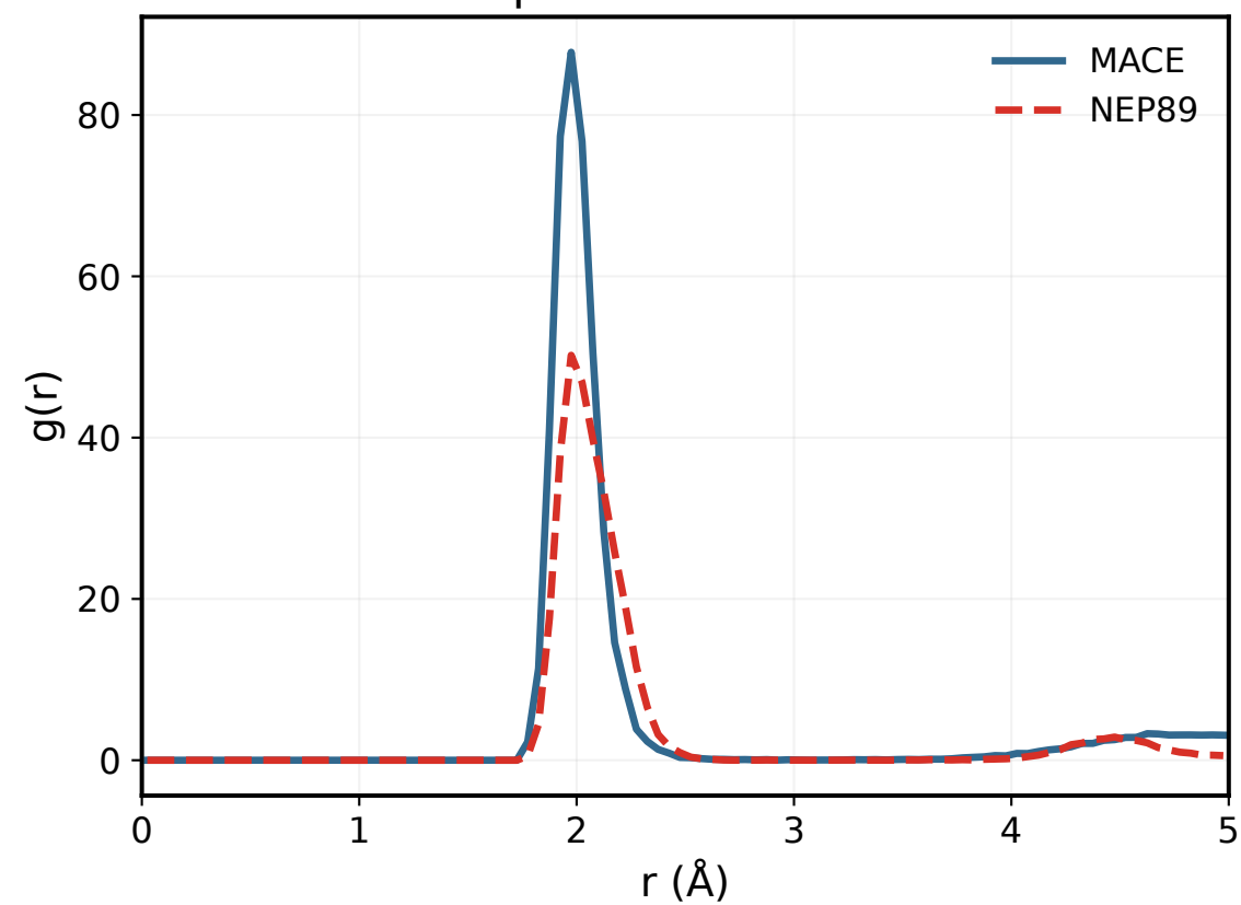
Zr-O partial RDF at 900 K
