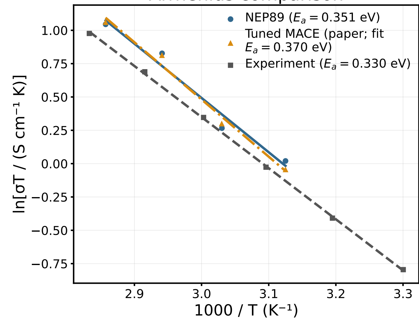
Arrhenius comparison
