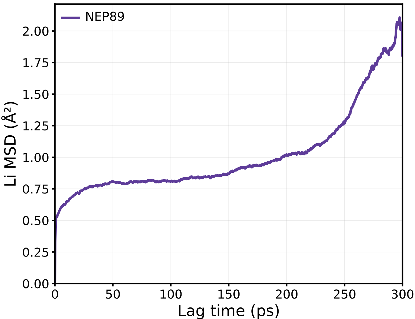
LSZC — 350 K
