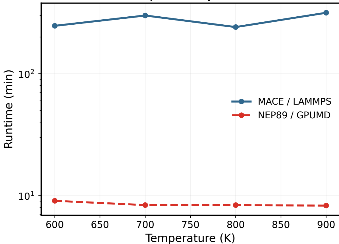
Four-temperature job runtimes
