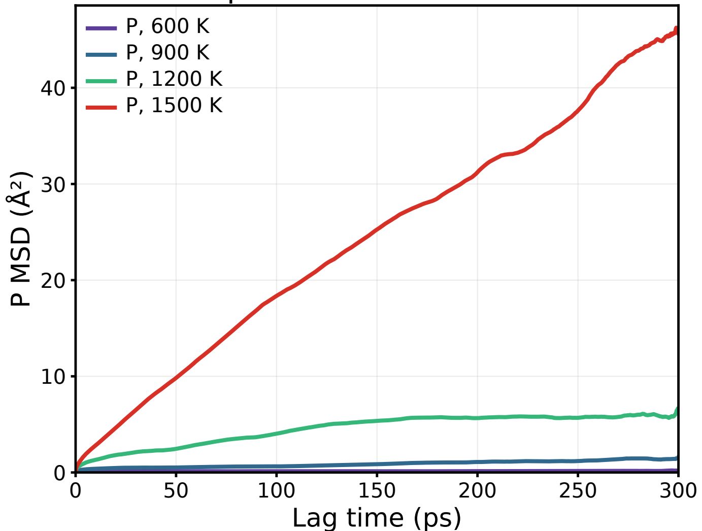
Phosphate-framework motion
