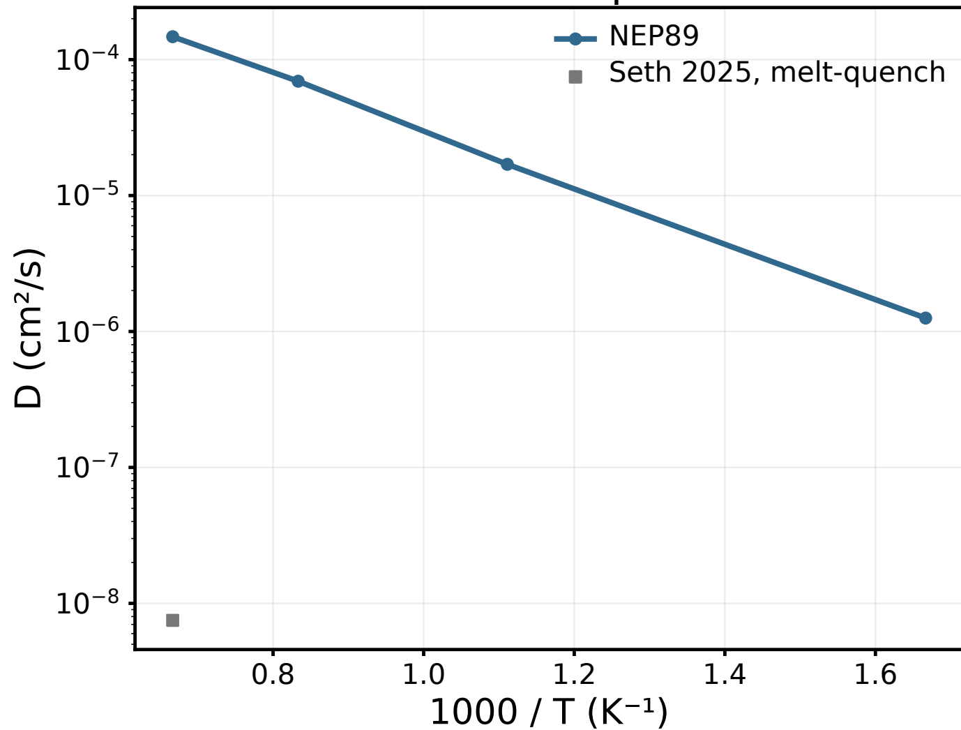
Bulk transport
