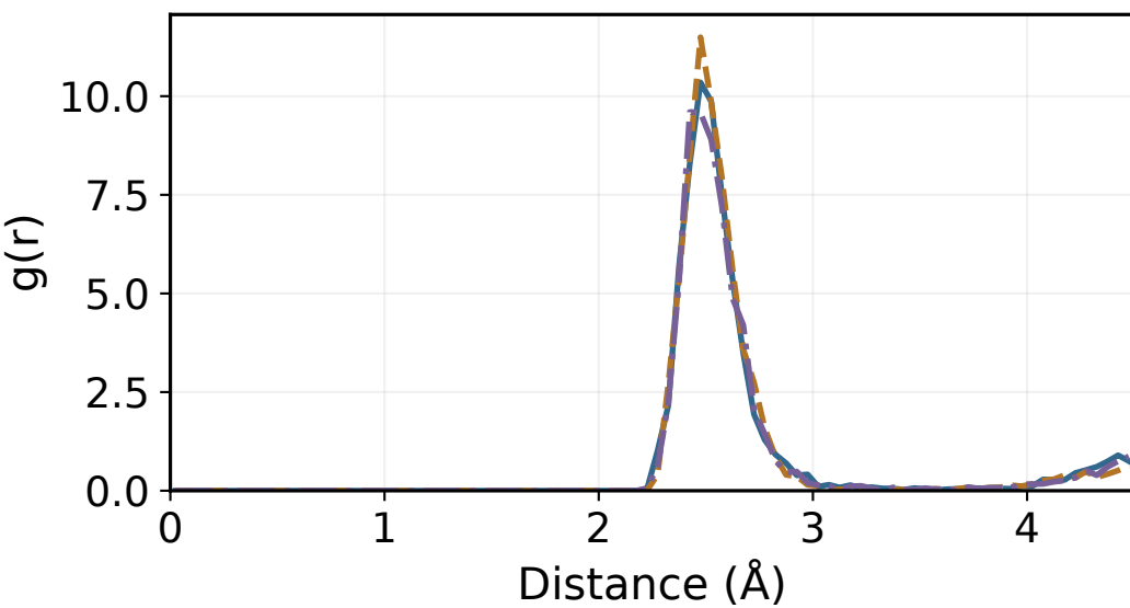
Zr-Cl
