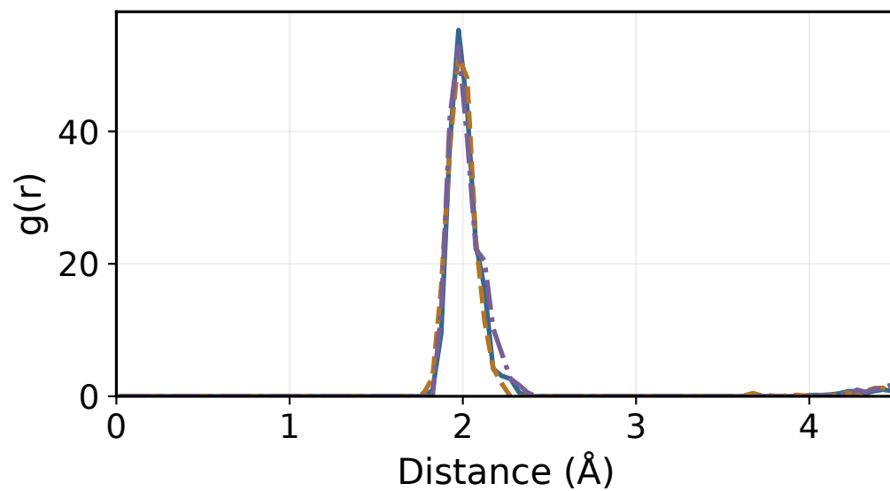
Zr-O
