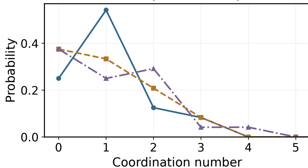
Zr-O (cutoff 2.6 Å)
