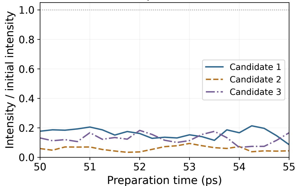
Cl initial-peak retention
