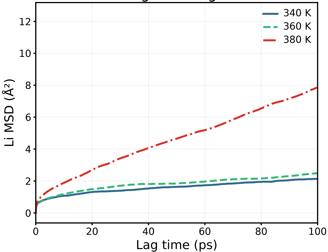
Time-origin averaged MSD
