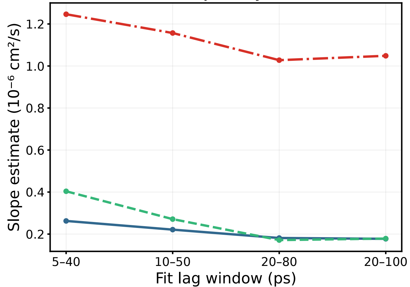
Window sensitivity (full trajectory)
