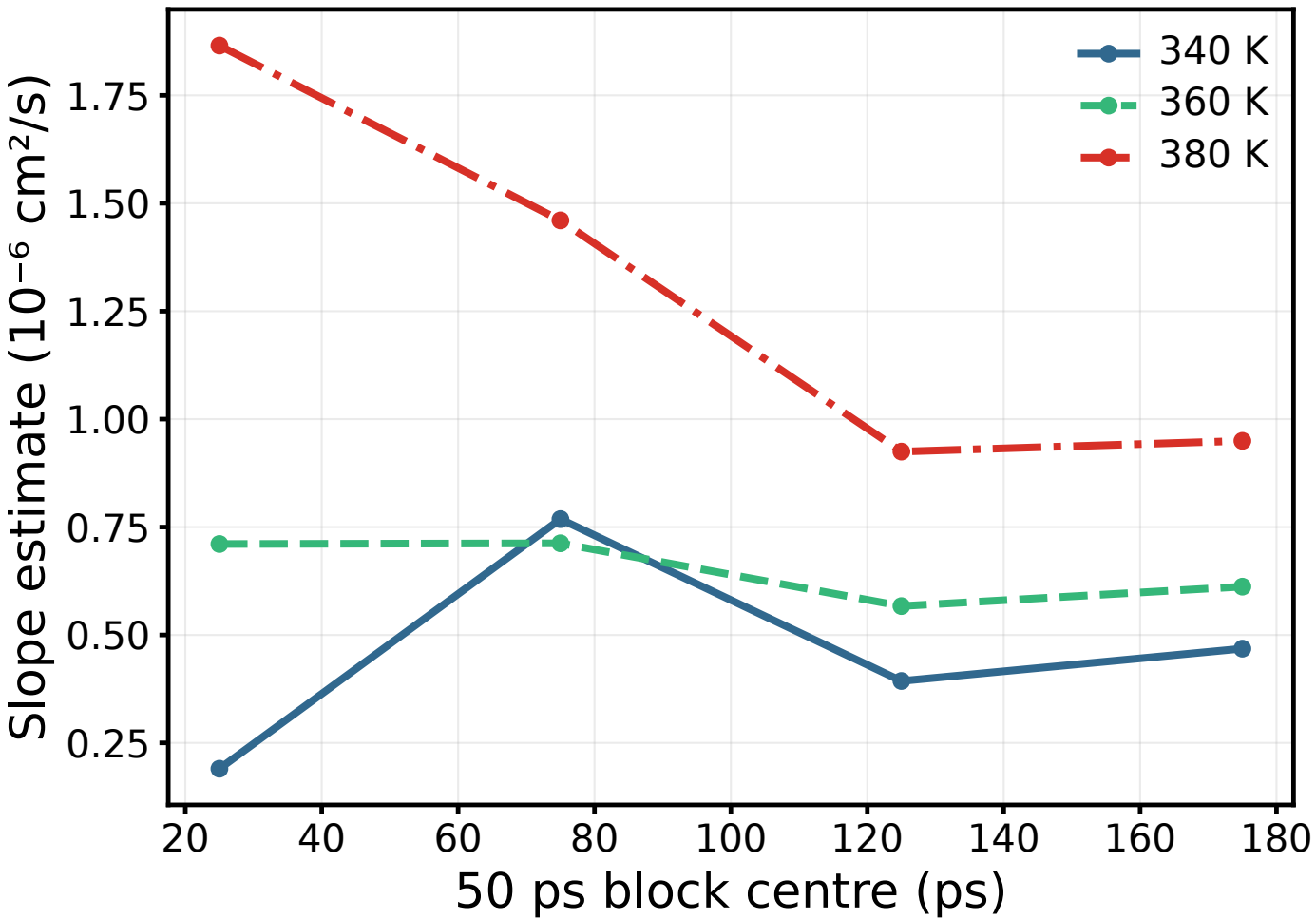
Within-trajectory blocks (5-20 ps fit)
