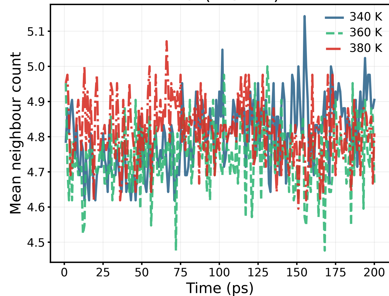
Zr-O ( < 2.6 \text{ \AA} )
