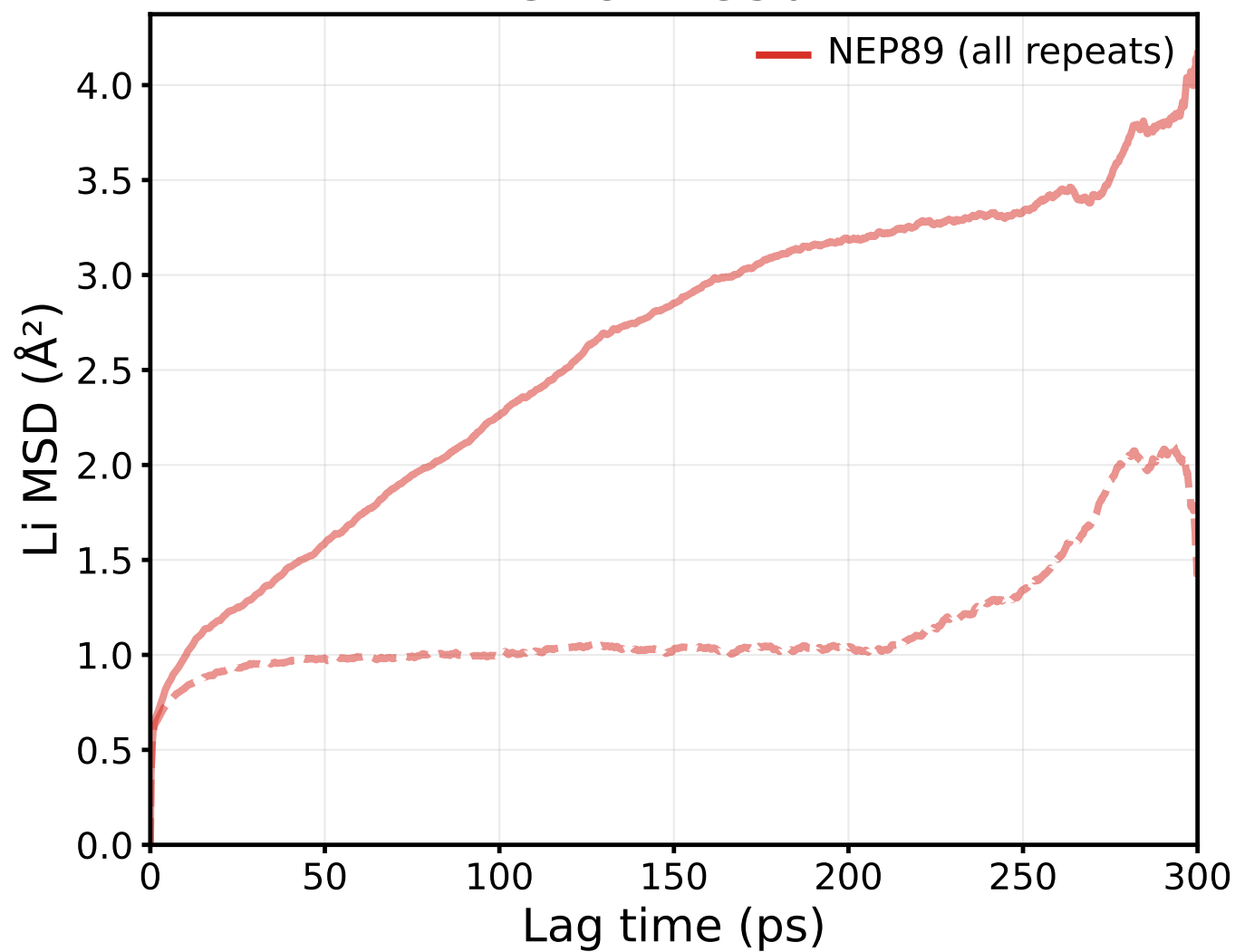
LSZC — 350 K
