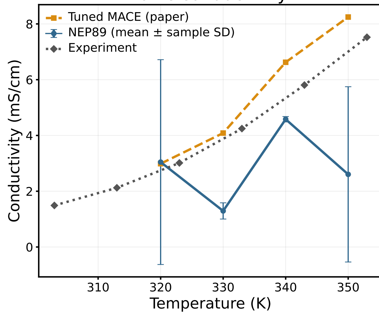
Ionic conductivity
