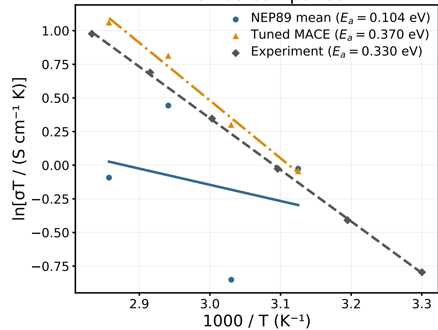
Arrhenius comparison
