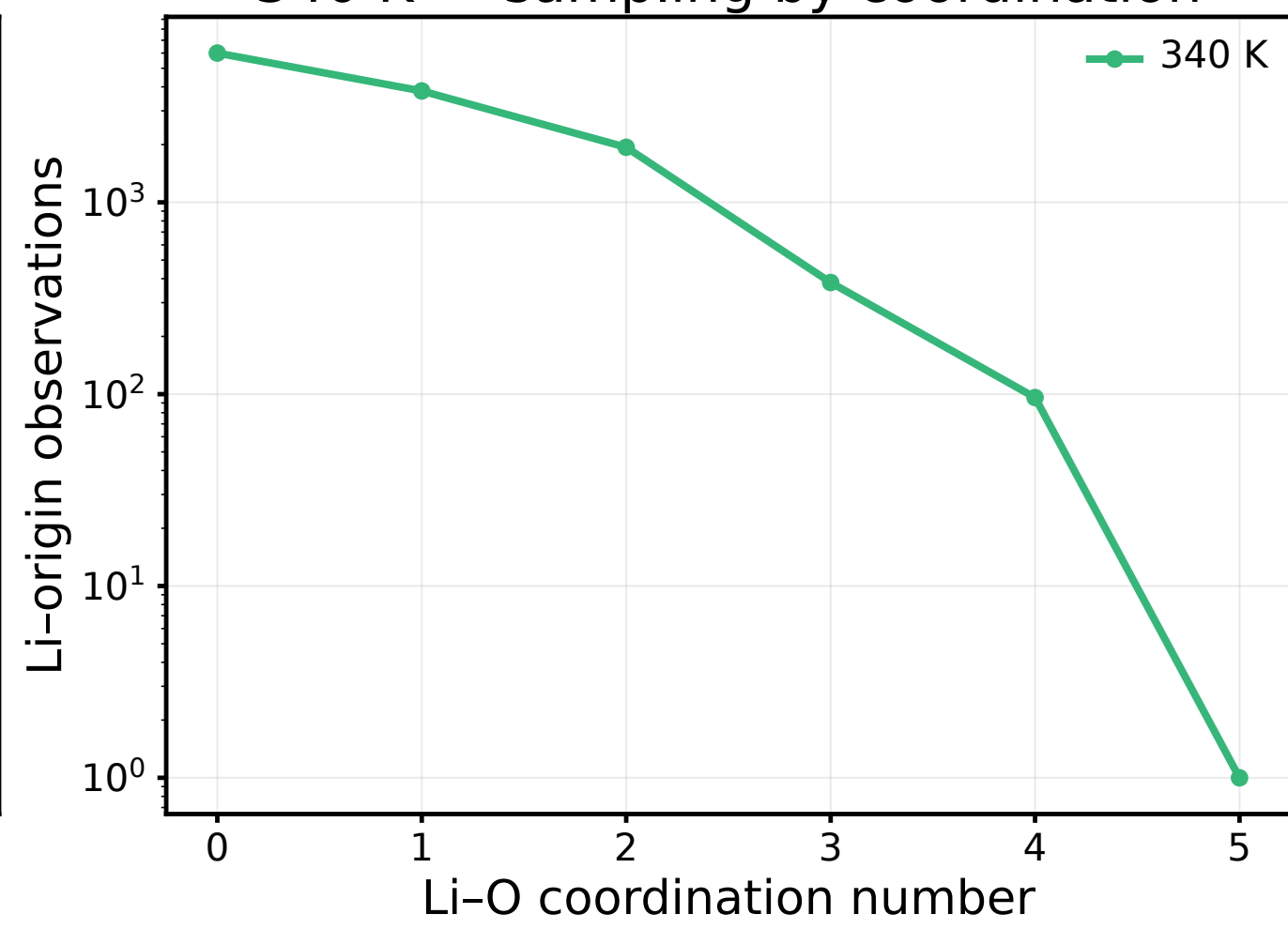
340 K — sampling by coordination
