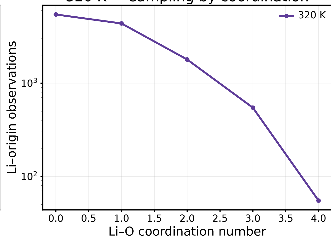
320 K — sampling by coordination
