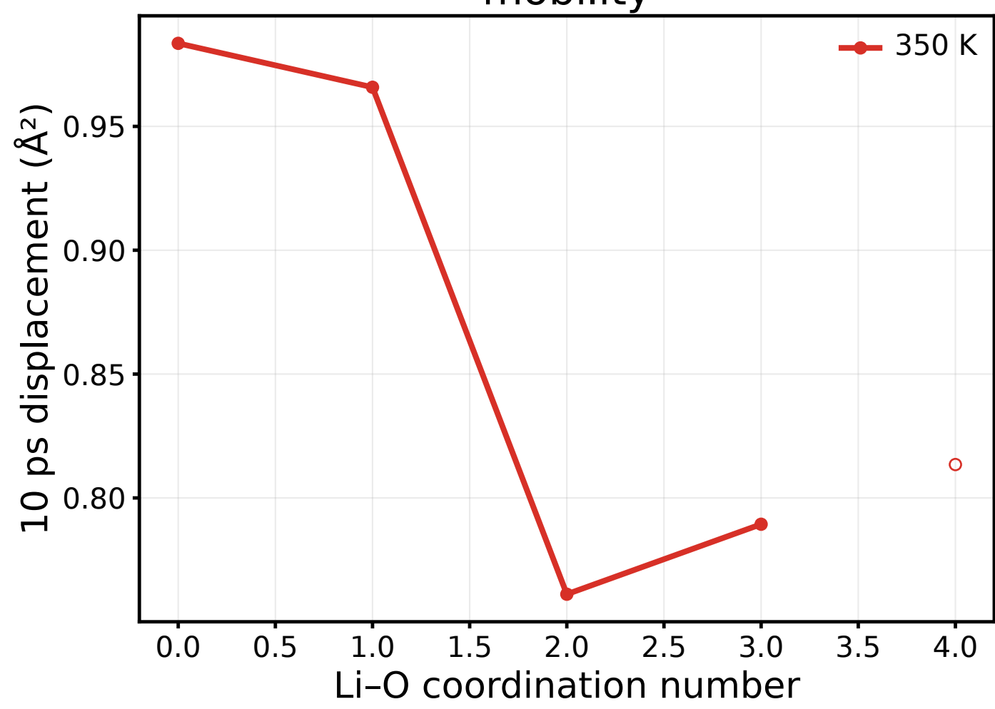
350 K — Li-O coordination and mobility
