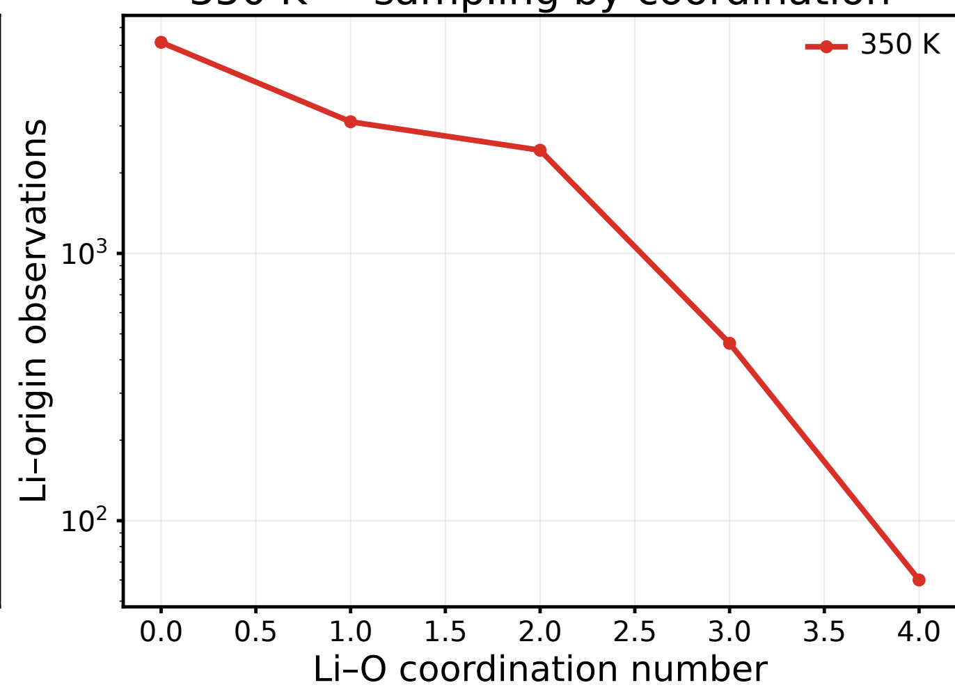
350 K — sampling by coordination
