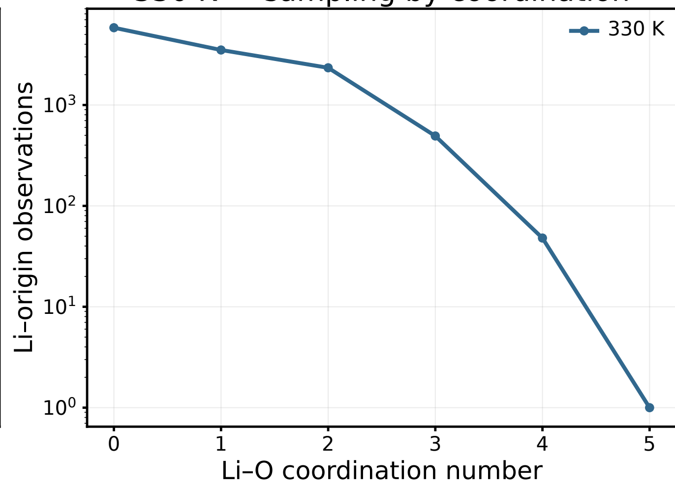
330 K — sampling by coordination
