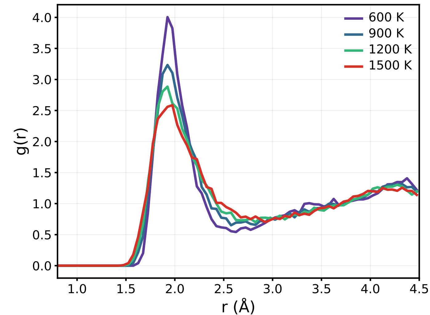
Li-O radial distribution
