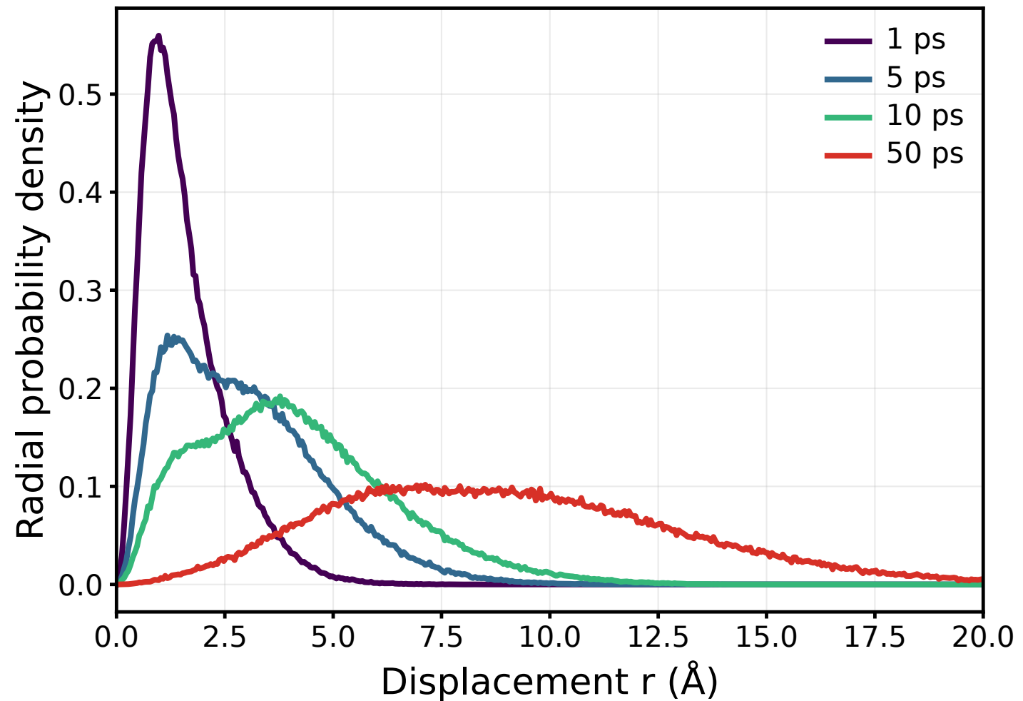
Li self van Hove distribution at 900 K
