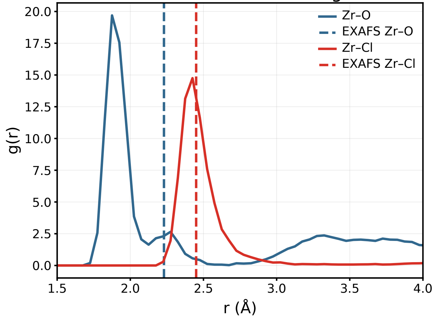
RDF and EXAFS bond lengths
