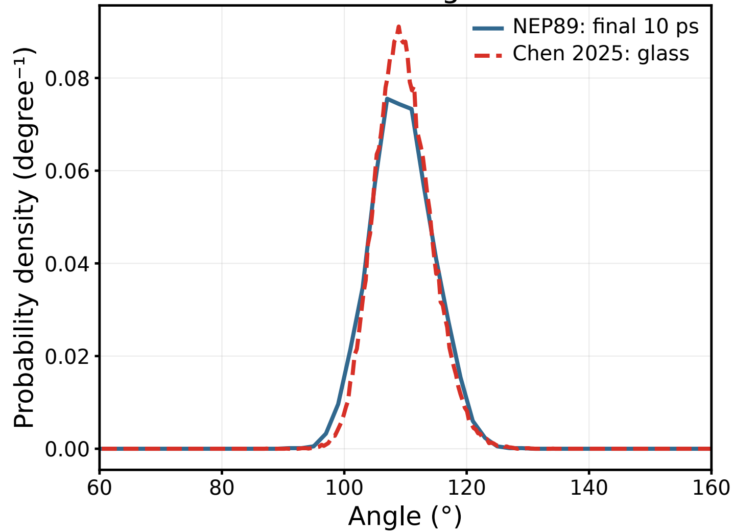
S-P-S angles
