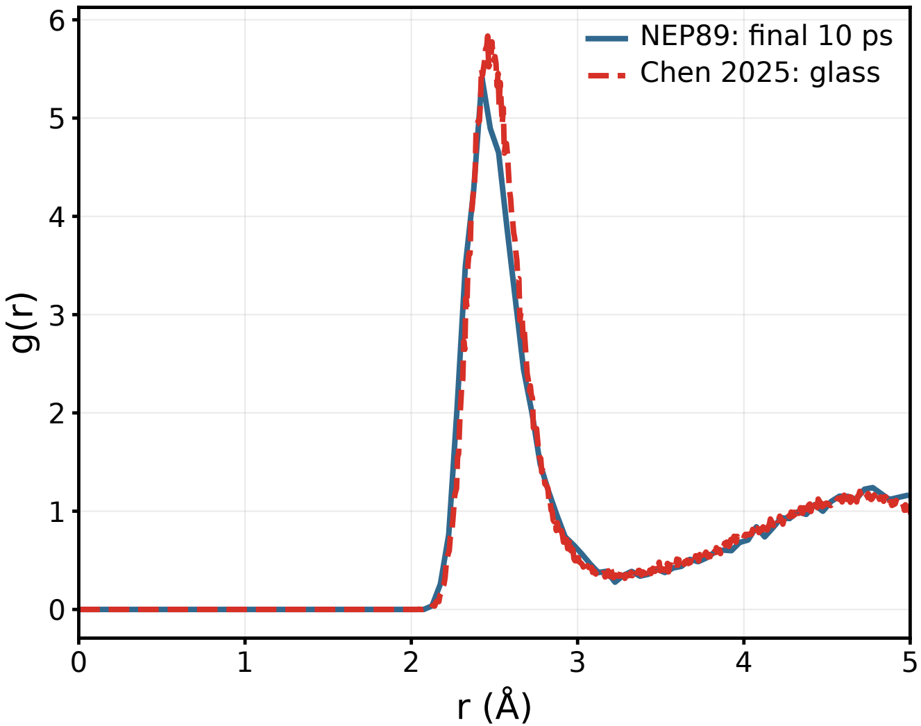
Li-S RDF
