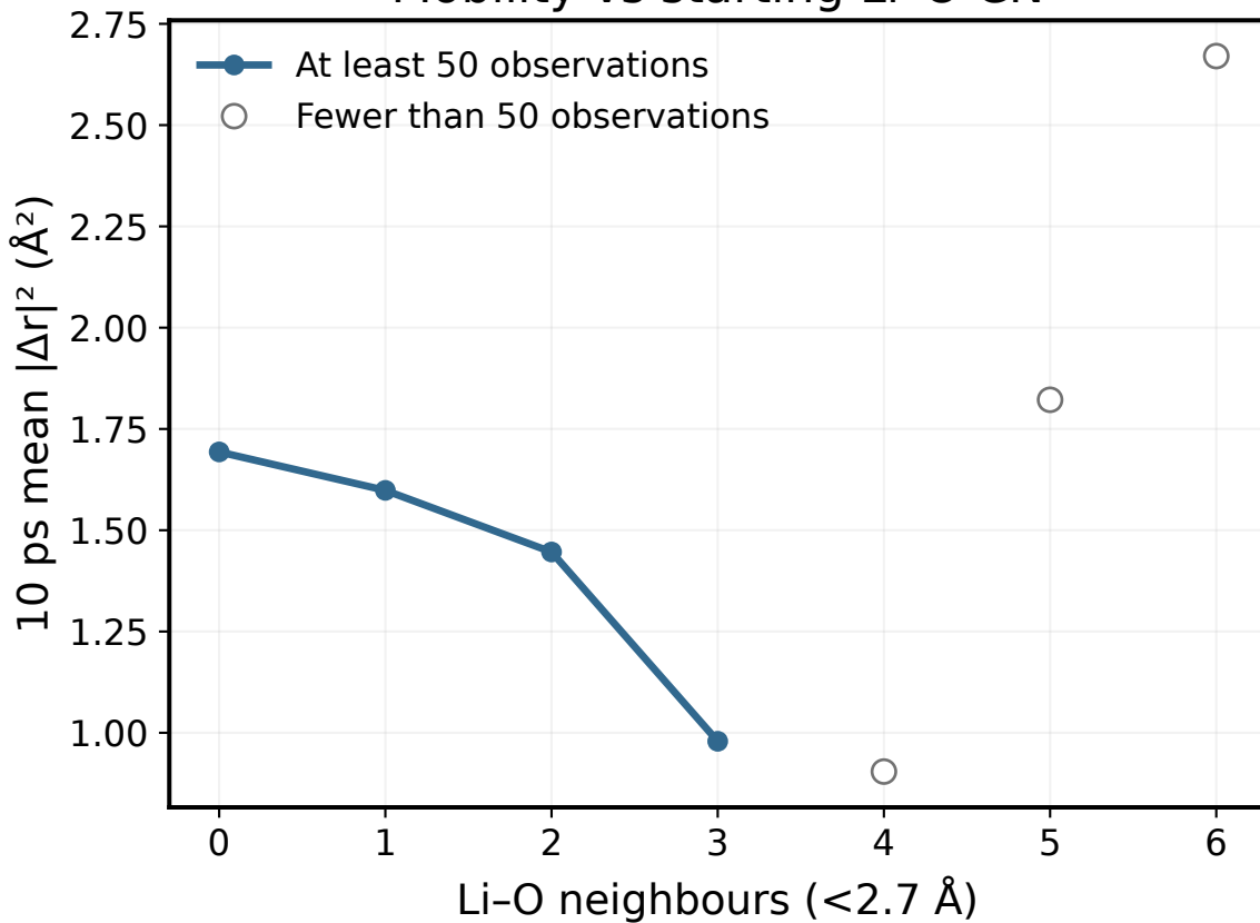
Mobility vs starting Li-O CN
