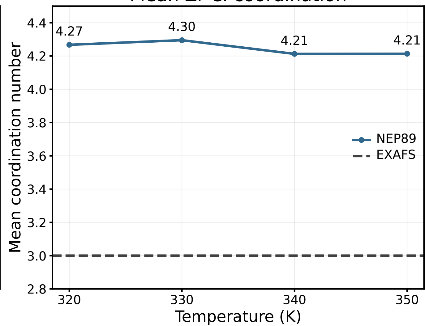
Mean Zr-Cl coordination
