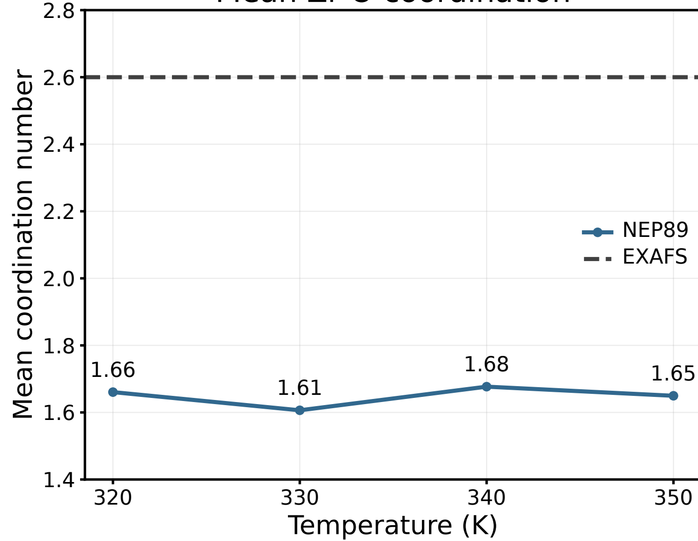
Mean Zr-O coordination
