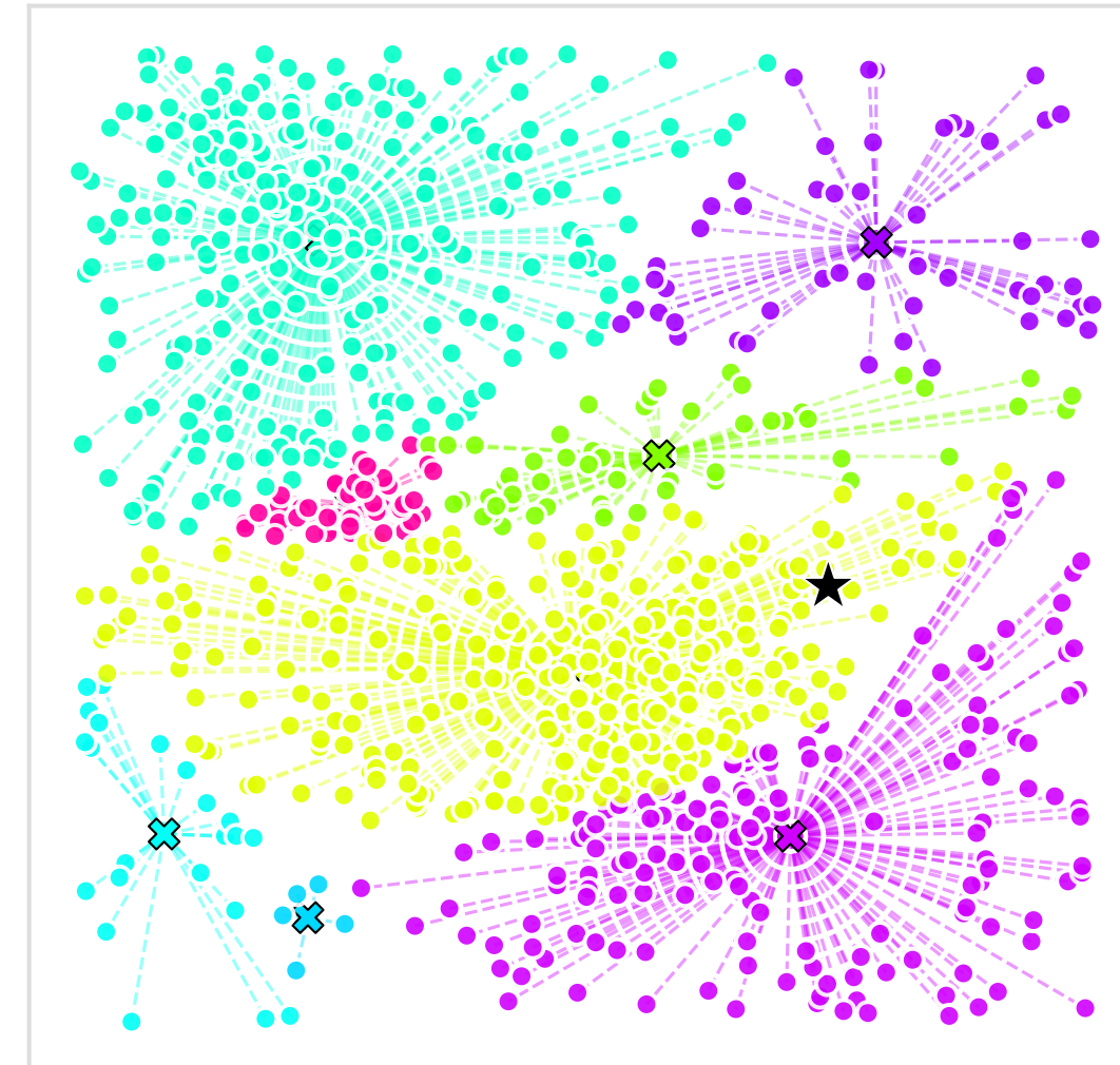
X-n957-k87 (Size 956)
