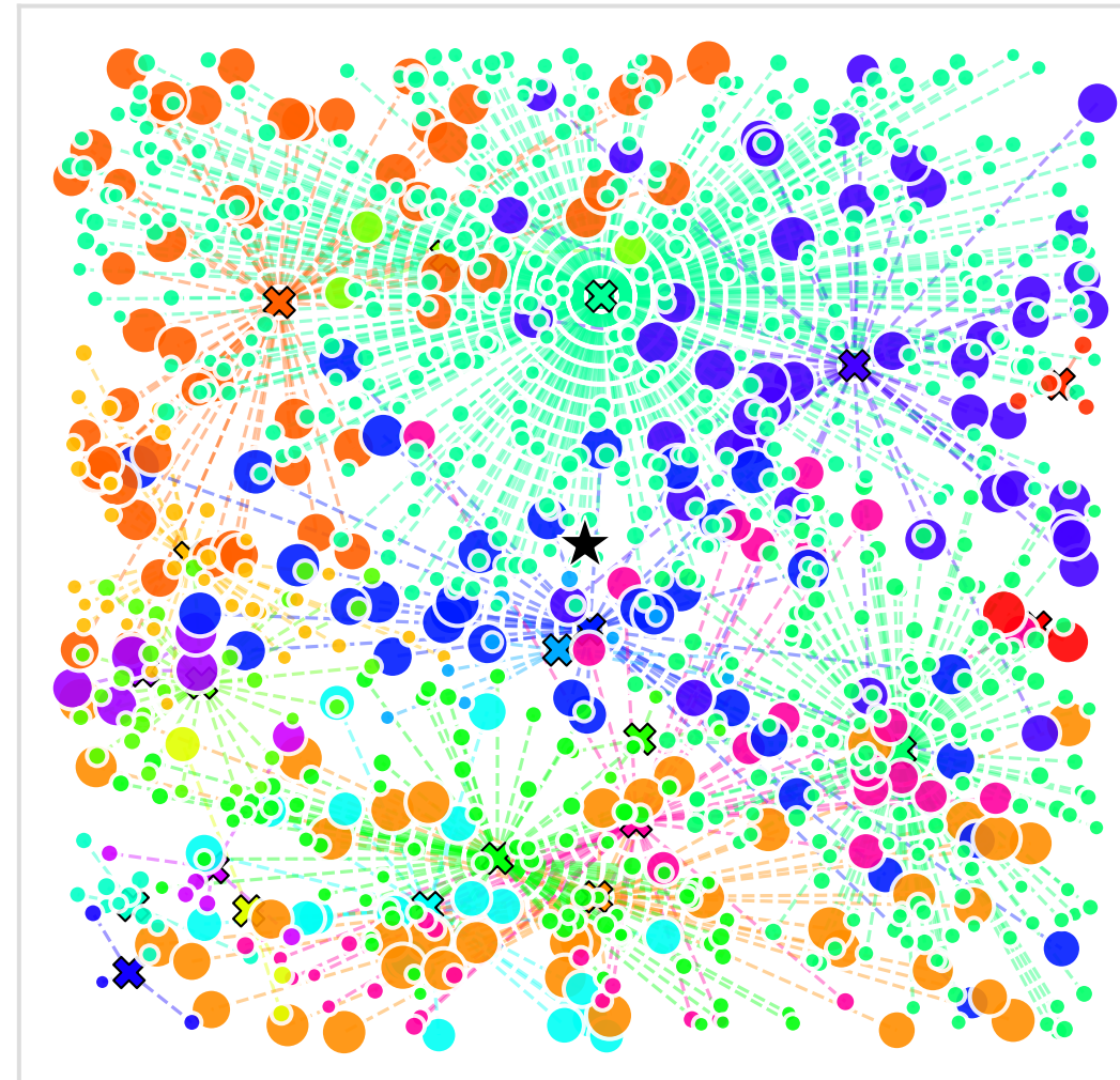
X-n936-k151 (Size 935)
