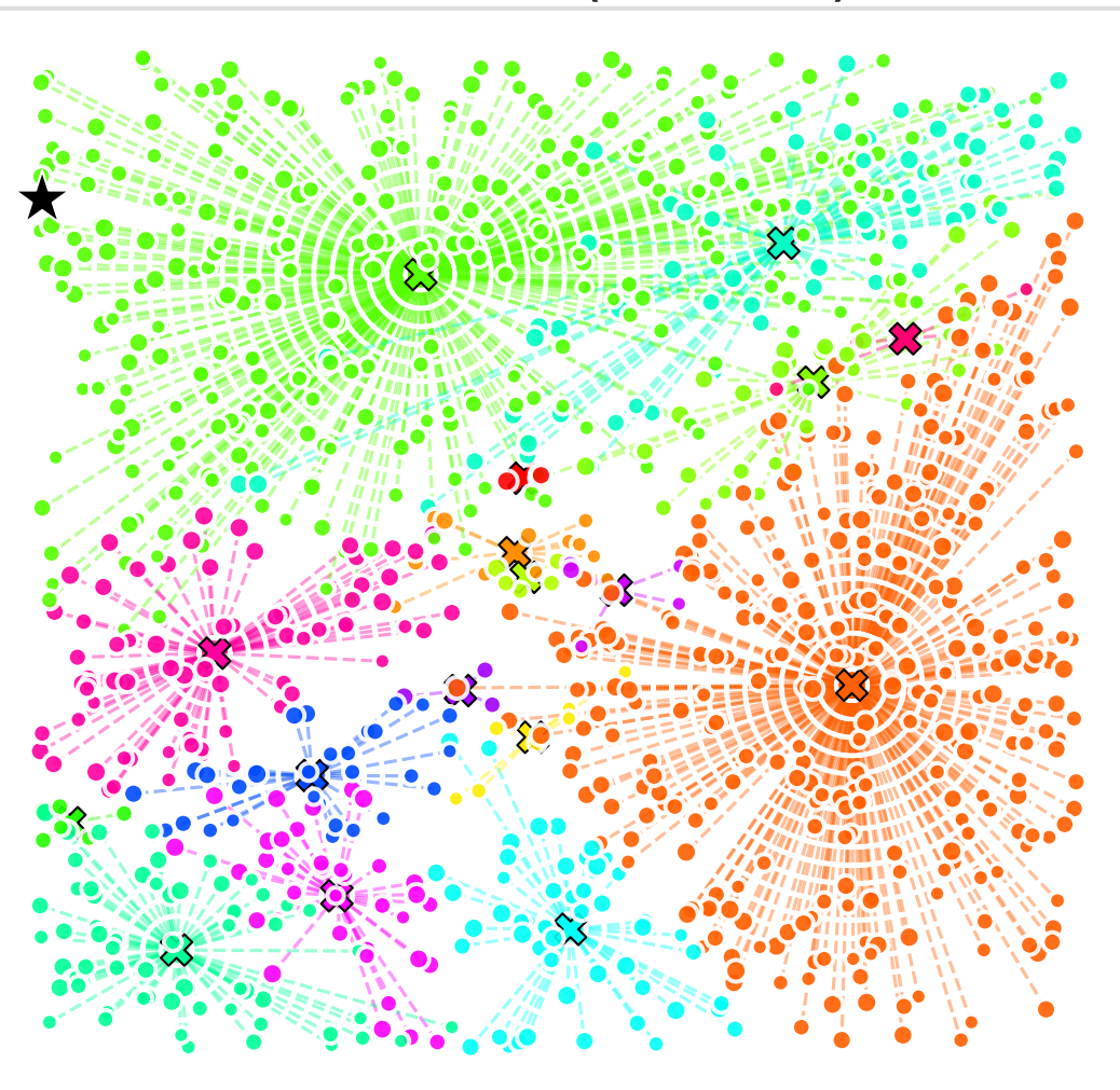
X-n1001-k43 (Size 1000)
