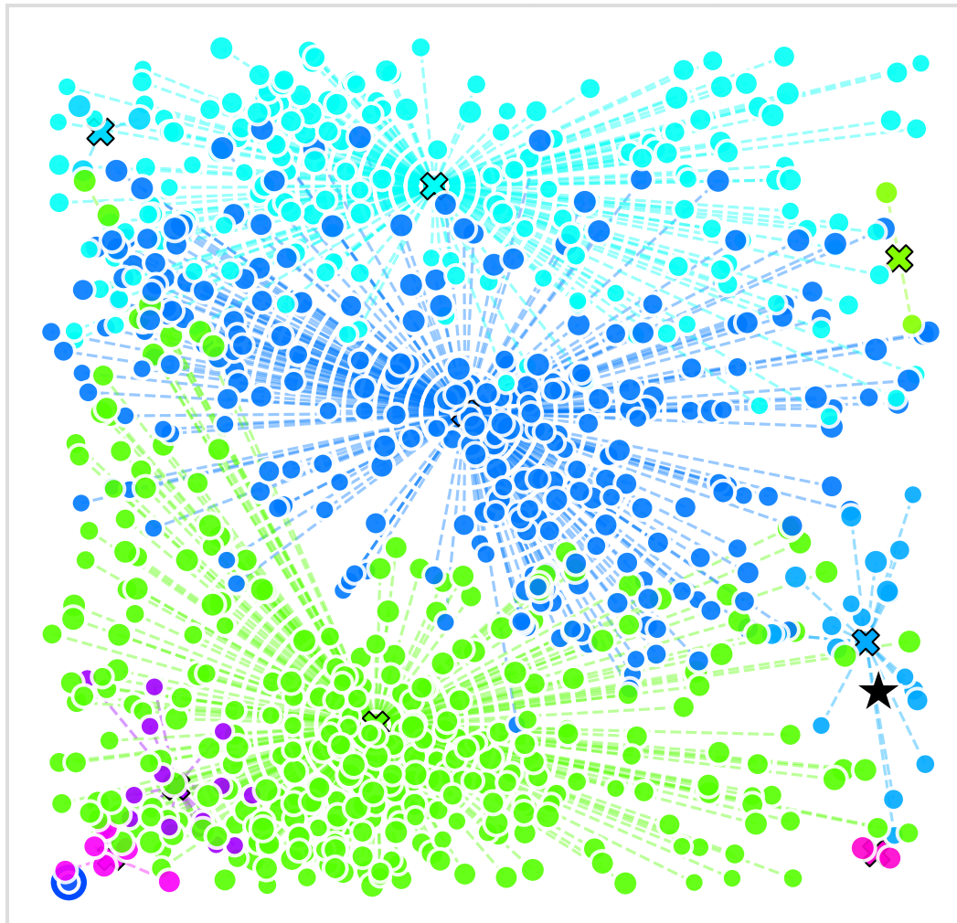
X-n837-k142 (Size 836)
