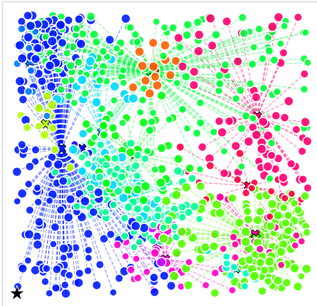
X-n916-k207 (Size 915)
