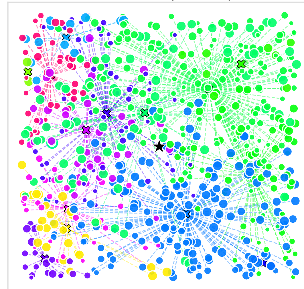
X-n733-k159 (Size 732)
