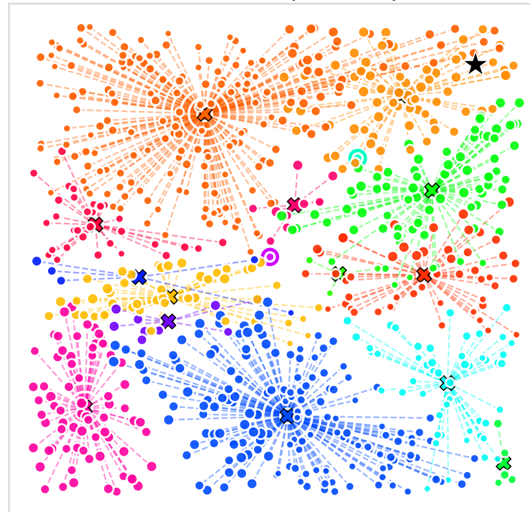
X-n783-k48 (Size 782)
