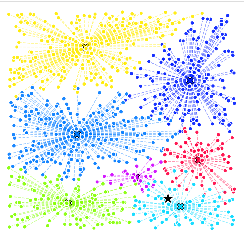
X-n895-k37 (Size 894)
