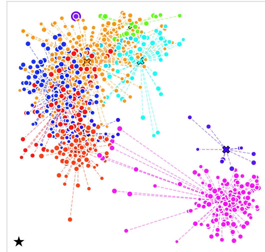
X-n876-k59 (Size 875)
