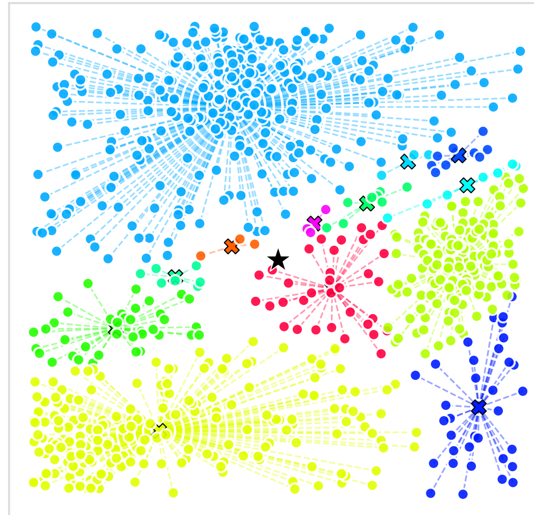
X-n856-k95 (Size 855)
