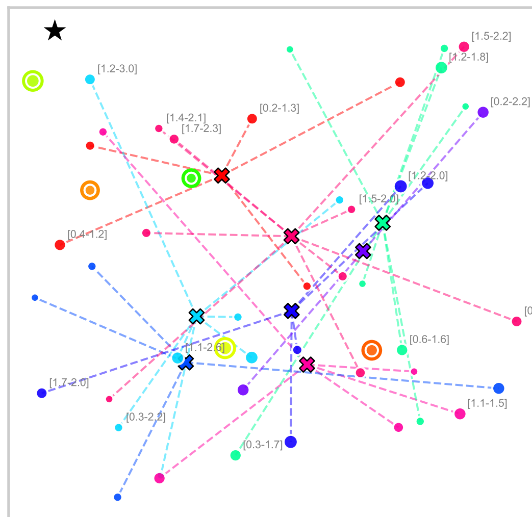
VRPTW
