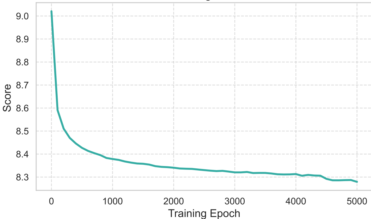
Score Convergence: VRPB
