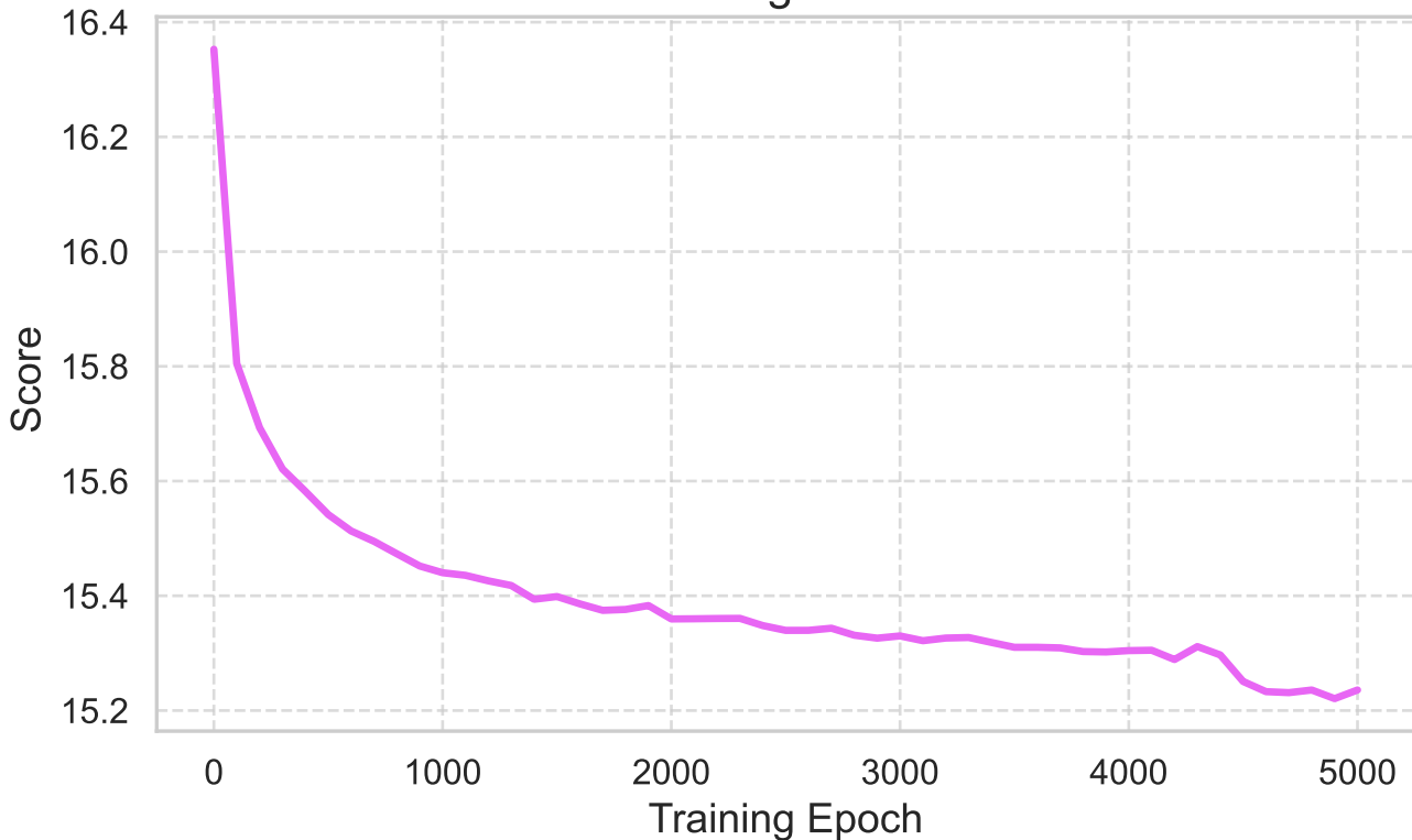
Score Convergence: VRPTW
