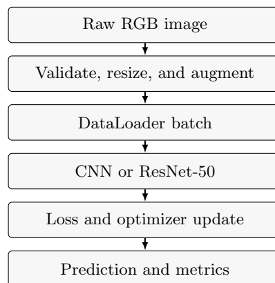
Figure 2: Planned Assignment 2 training and evaluation pipeline.
