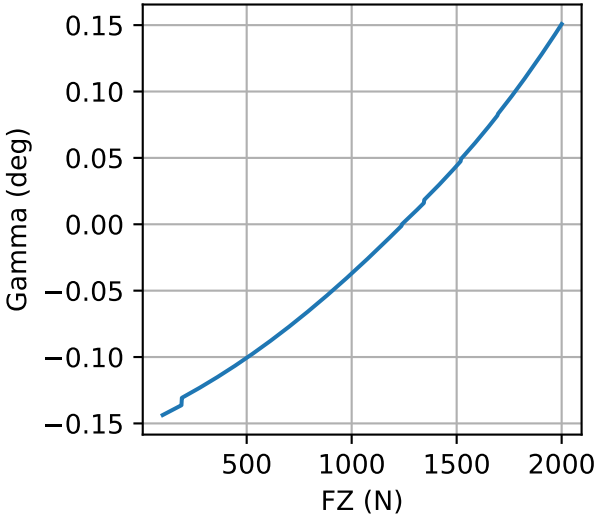
Gamma at Peak Fy vs Fz
