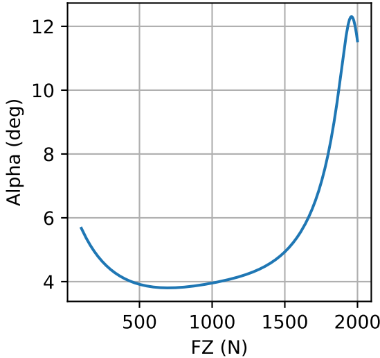
Peak Mz Alpha vs FZ
