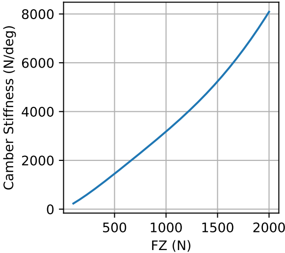
Camber Stiffness vs FZ
