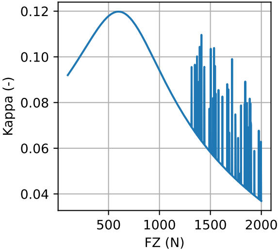
Peak Fx Kappa vs FZ
