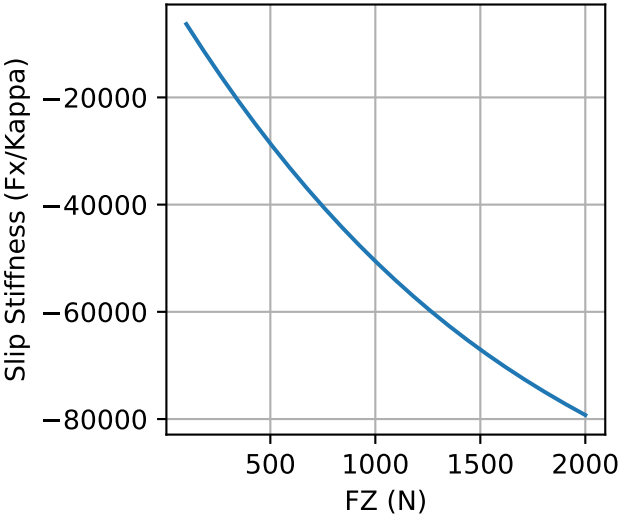
Slip Stiffness vs FZ
