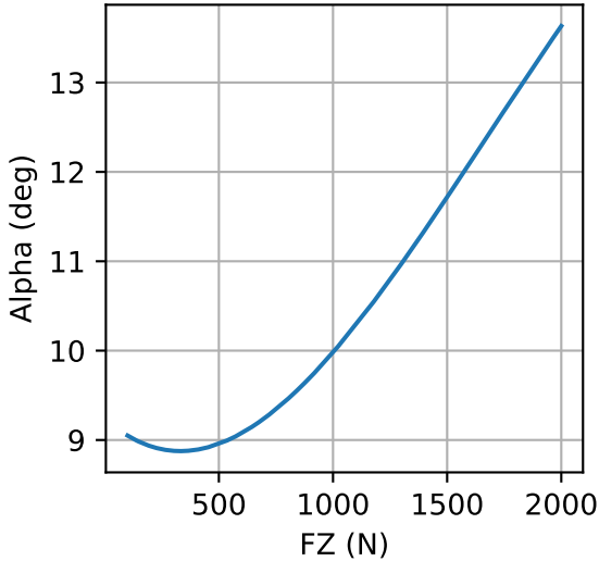
Peak Fy Alpha vs FZ
