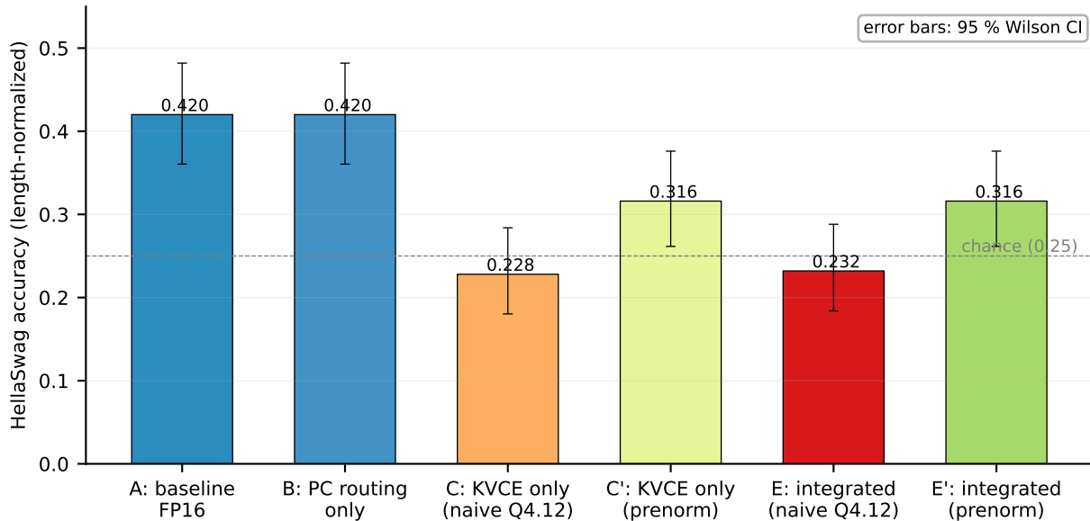
Qwen2-0.5B HellaSwag (val, n=250)
