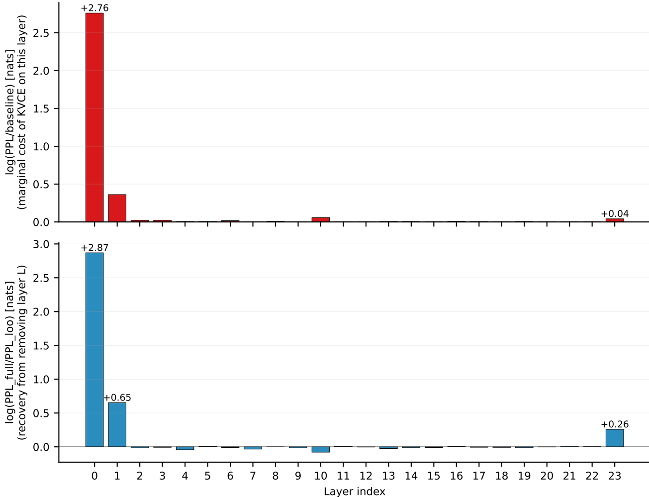
Per-layer KVCE cost on Qwen/Qwen2-0.5B (mode=C_prenorm, n=16 chunks, PPL_A=21.06, PPL_full=119.9)
