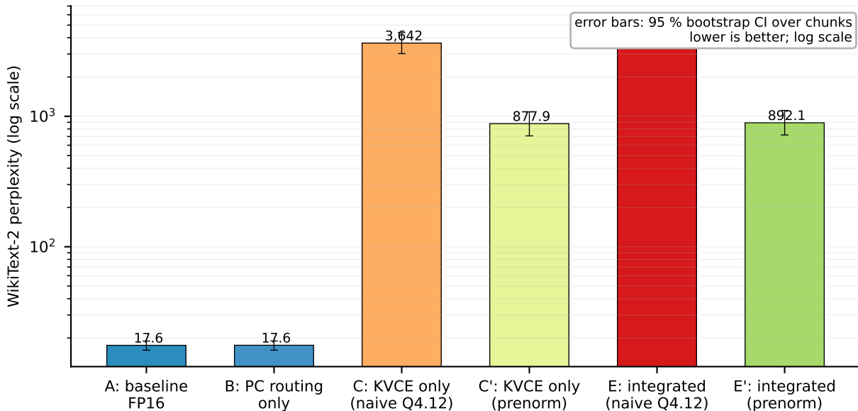
Qwen2-0.5B WikiText-2 perplexity, ACU x KVCE attention substitute (64 x 512-token chunks)
