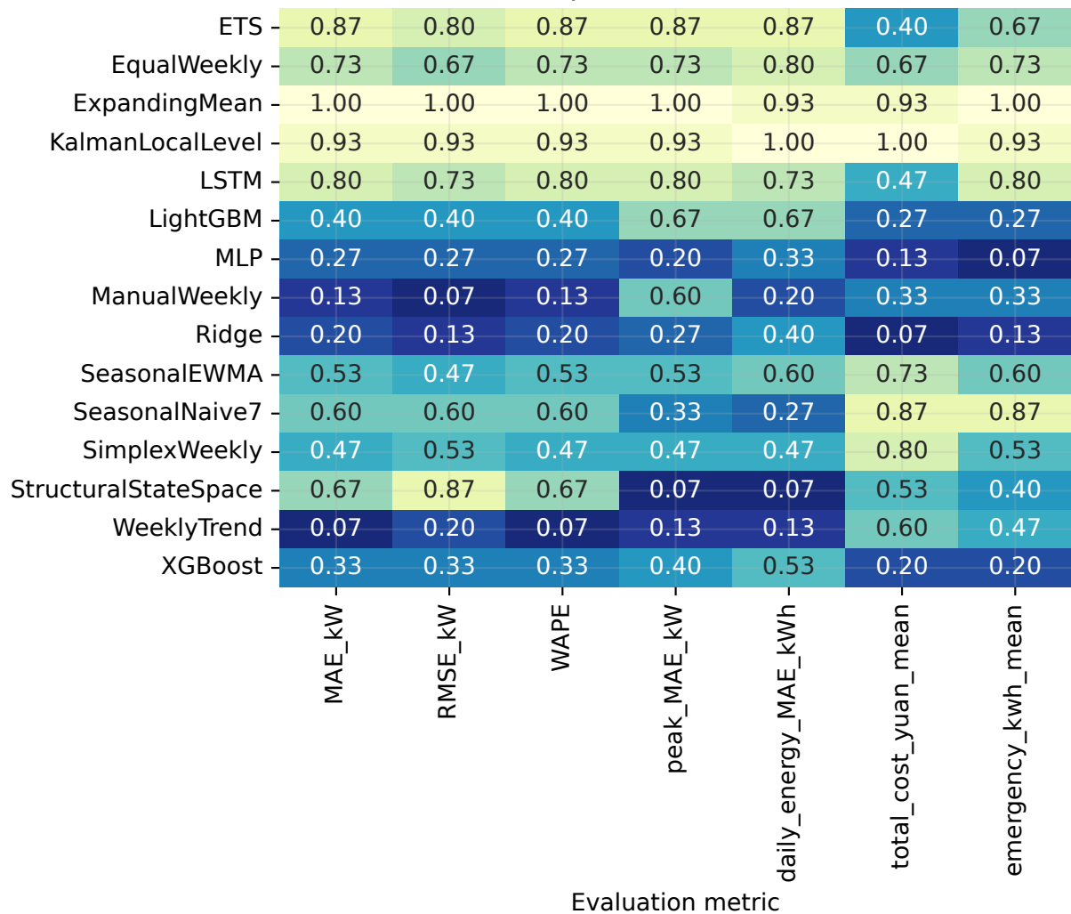
(a) Multi-metric comparison
