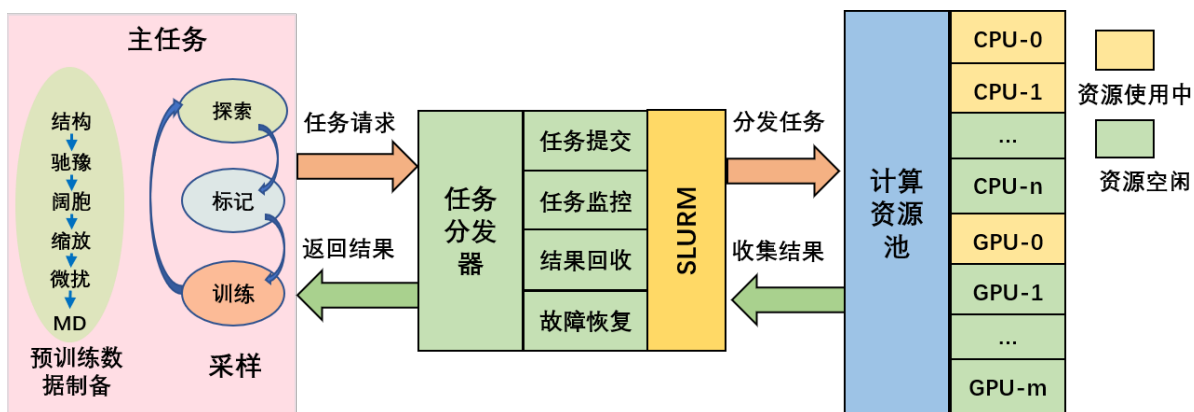
Figure 13: PWact platform architecture
