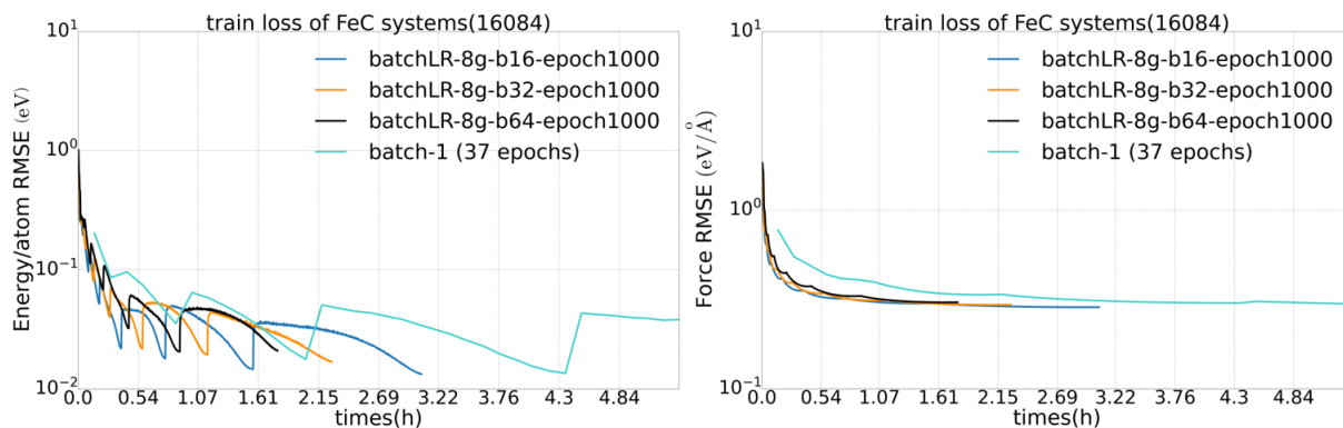
Figure 4: NEP training on the FeC dataset
