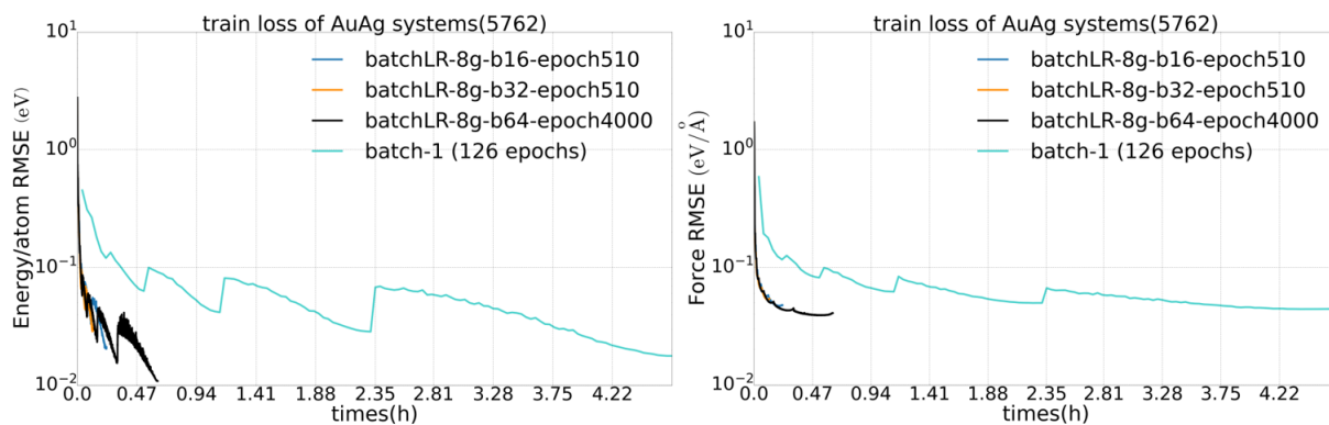
Figure 5: NEP training on the AuAg dataset
