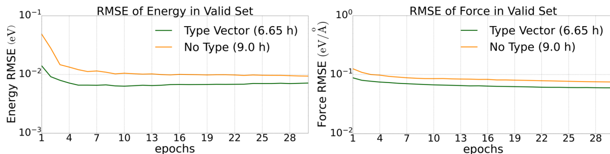
Figure 7: Reduction in energy and force errors on the validation set for the five-component alloy system
