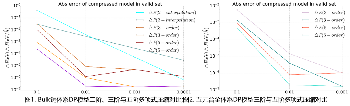
Figure 11: Accuracy comparison for different model-compression orders
