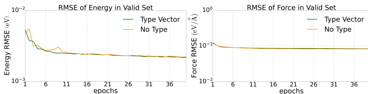
Figure 8: Reduction in energy and force errors on the validation set for the quaternary LiGePS system
