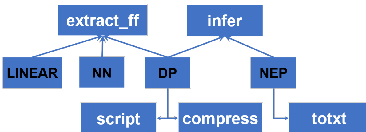
Figure 1: MatPL utility commands
