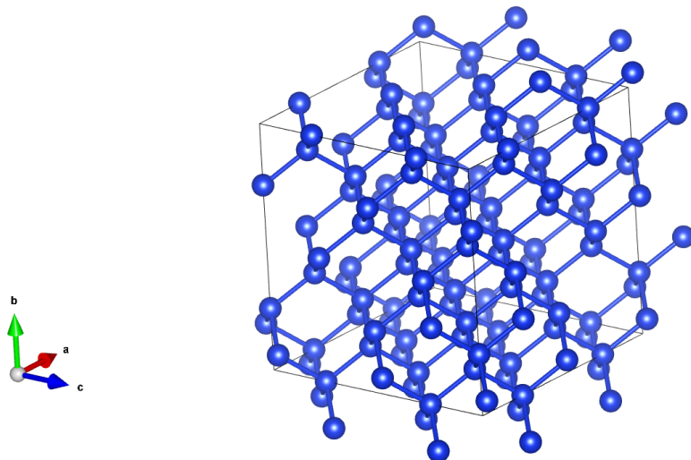
Figure 16: 硅体相
