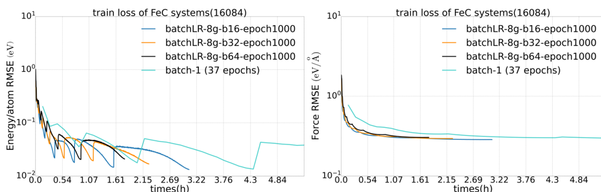
Figure 4: NEP training on the FeC dataset
