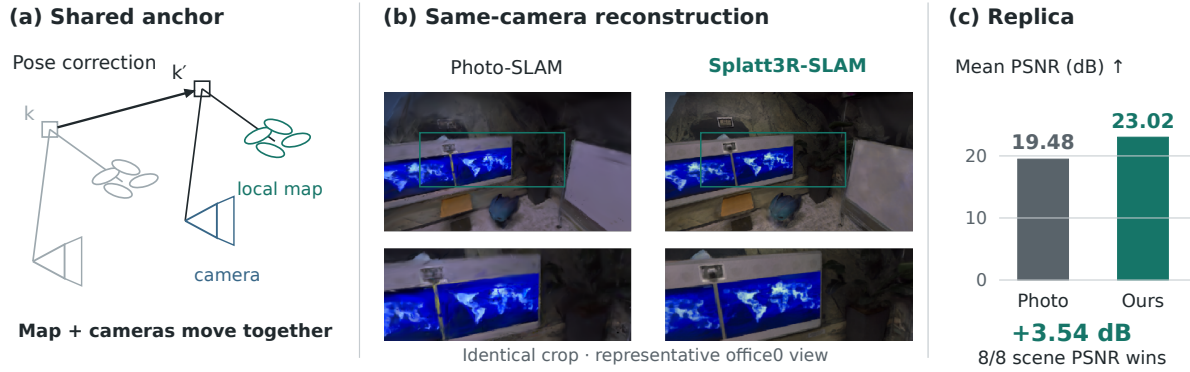
Figure 1.1. (a) Shared keyframe anchors move local Gaussians and their observation cameras together after pose corrections; grey shows their previous positions. (b) Common-camera renderings with identical crops. (c) On eight Replica scenes, Splatt3R-SLAM reaches 23.02 dB after 300 s polish, exceeds Photo-SLAM by 3.54 dB, and leads PSNR on every scene.
