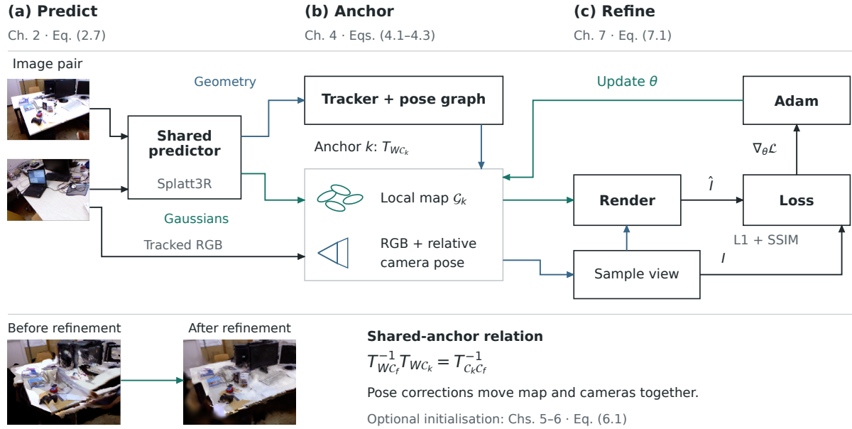
Figure 4.1. Method navigation. Real input frames enter a shared predictor. Geometry feeds tracking, while local Gaussians attach to keyframe anchors. The same anchors carry supervision cameras. A separate process samples observations, renders the map, and updates its appearance. Insets show saved maps before and after refinement. Chapter and equation labels point to the detailed derivation.
