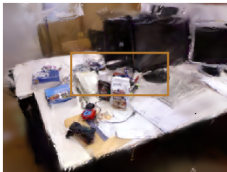
Photo-SLAM
