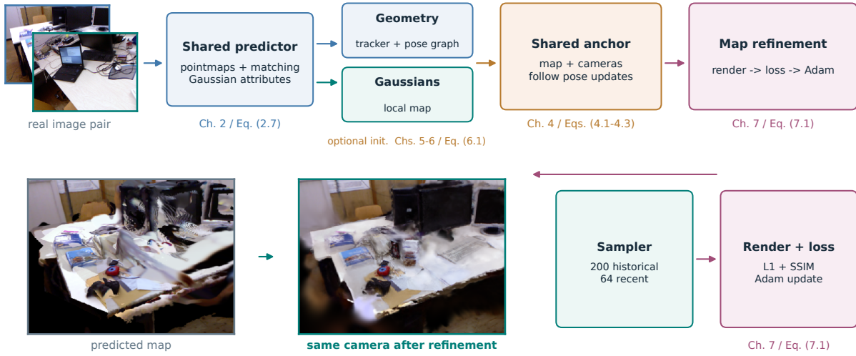
Figure 4.1. Method navigation. Real input frames enter a shared predictor. Geometry feeds tracking, while local Gaussians attach to keyframe anchors. The same anchors carry supervision cameras. A separate process samples observations, renders the map, and updates its appearance. Insets show saved maps before and after refinement. Chapter and equation labels point to the detailed derivation.
