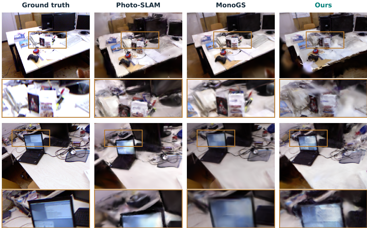
Figure 9.3. Ground truth, Photo-SLAM, MonoGS and Ours, at two common TUM desk cameras. Each full view is followed by an identical crop, indicated in orange. Views occupy the two middle ranks of Ours-minus-MonoGS per-frame PSNR. Remaining blur and geometric distortion are visible in both MonoGS and our maps. No per-image score labels are used.
