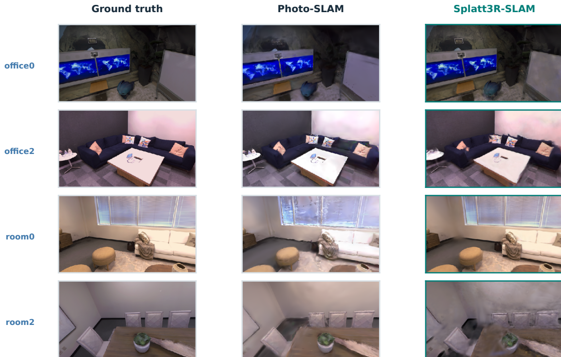
Figure 9.1. Ground truth, Photo-SLAM, and Splatt3R-SLAM on four Replica scenes. Each row uses one common evaluation camera. MonoGS is absent because no comparable monocular Replica map was available.
