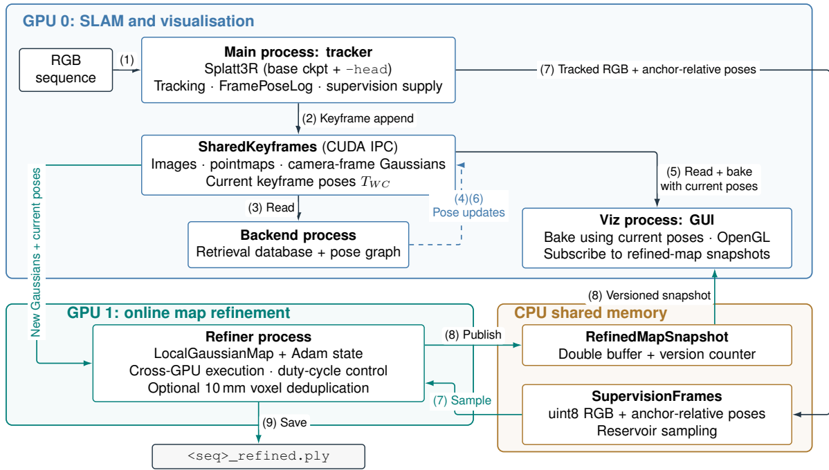
Figure 4.2. System implementation. Tracking, backend optimisation, and visualisation run on GPU 0; the map refiner runs on GPU 1. SharedKeyframes uses CUDA IPC, while supervision frames and versioned refined-map snapshots use CPU shared memory. Numbered arrows show data flow and pose updates.
