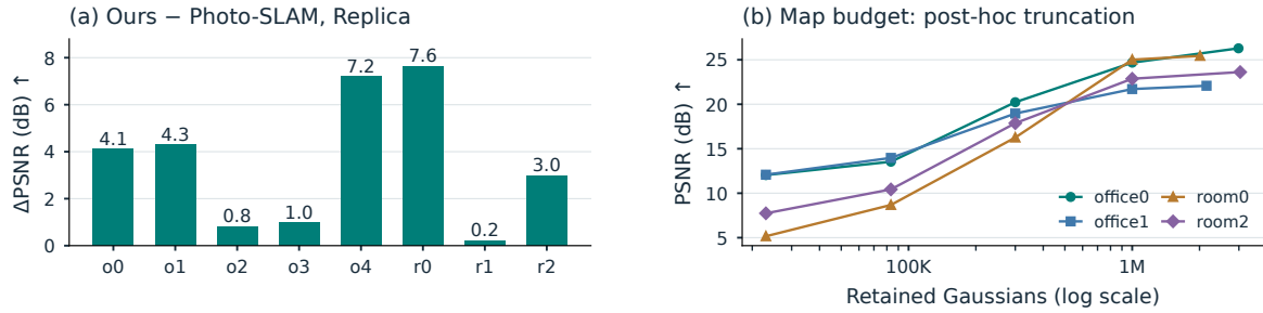
Figure 9.2. (a) Fresh full-SH Replica scene PSNR differences; o/r denote office/room. (b) A separate recorded experiment retaining the highest-opacity primitives in four of our maps, without re-optimisation. Final markers denote full maps. The truncation curve measures sensitivity to this procedure, not optimal quality under each primitive budget.
