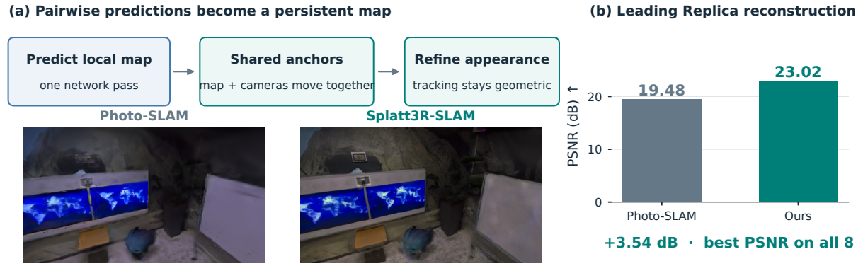
Figure 1.1. Shared keyframe anchors move local Gaussians and their observation cameras together after pose corrections, while a separate process refines appearance. On eight Replica scenes, Splatt3R-SLAM reaches 23.02 dB, exceeds Photo-SLAM by 3.54 dB, and establishes state-of-the-art performance.
