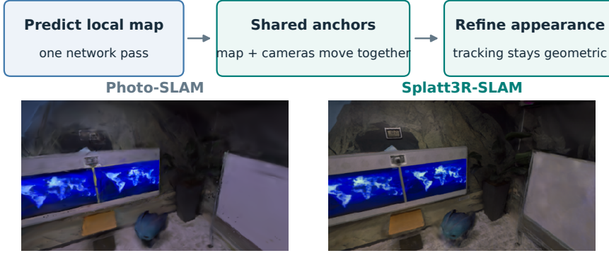
Fig. 1. Pairwise predictions become a persistent map. Shared keyframe anchors move local Gaussians and their observation cameras together after pose corrections, while a separate process refines appearance. On eight Replica scenes, Splatt3R-SLAM reaches 23.02 dB, exceeds Photo-SLAM by 3.54 dB, and leads PSNR on every scene. Results use common non-keyframe cameras and full exported SH.
