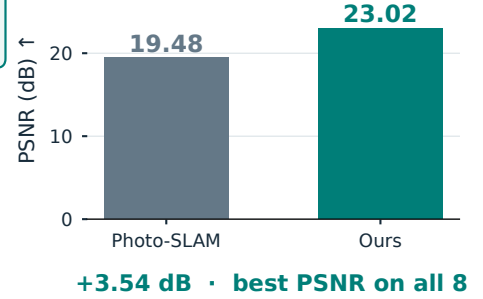
Fig. 1. Pairwise predictions become a persistent map. Shared keyframe anchors move local Gaussians and their observation cameras together after pose corrections, while a separate process refines appearance. On eight Replica scenes, Splatt3R-SLAM reaches 23.02 dB, exceeds Photo-SLAM by 3.54 dB, and leads PSNR on every scene. Results use common non-keyframe cameras and full exported SH.
