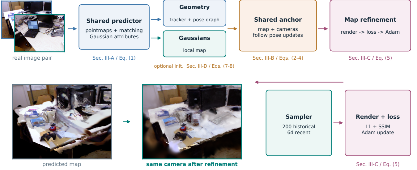
Fig. 2. Predict, anchor, refine. Real TUM frames enter a shared predictor. Its geometric outputs support tracking; its Gaussian outputs form local maps. A keyframe anchor carries each local map and its supervision cameras, so both follow pose corrections. The refiner samples tracked images, renders the assembled map, and updates Gaussian appearance. Section and equation references locate each step. Insets show saved maps before and after refinement at the same camera.
