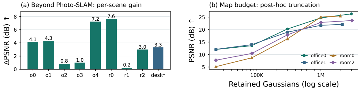
Figure 9.2. (a) Per-scene PSNR improvement over Photo-SLAM. Teal bars are Replica scenes (synthetic); the blue bar is real TUM desk at +3.3 dB. Gains range from +0.2 to +7.6 dB and are scene dependent. (b) Post-hoc truncation of four maps to their highest-opacity primitives without re-optimisation; quality falls off below about one million Gaussians, the final marker denoting each full map.
