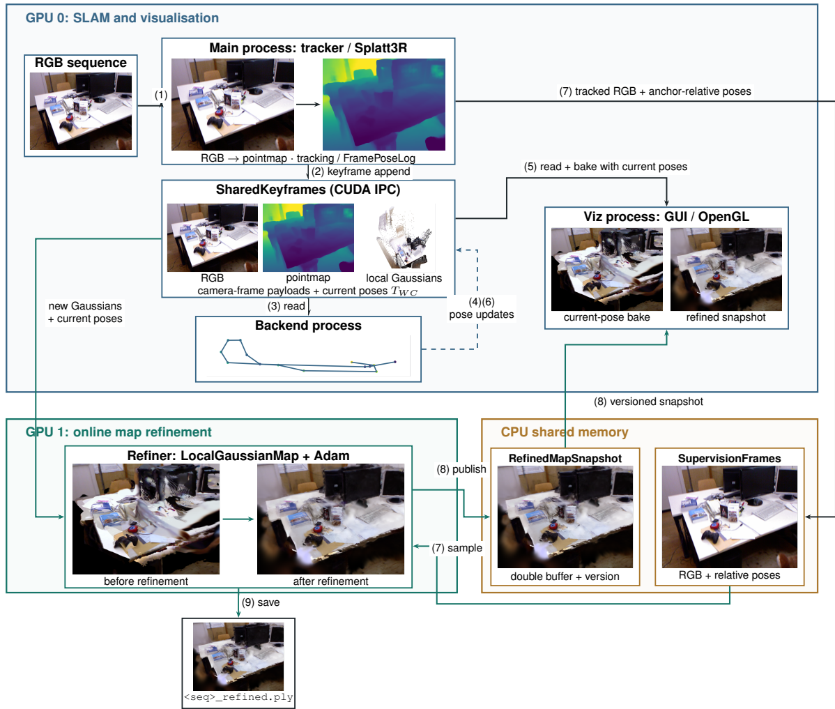
Figure 4.2. System overview. Tracking, backend optimisation, and visualisation run on GPU 0; the map refiner runs on GPU 1. SharedKeyframes uses CUDA IPC, while supervision frames and versioned refined-map snapshots use CPU shared memory. Numbered arrows show RGB, predicted pointmaps, local Gaussians, supervision and refined-map flow; dashed arrows denote pose updates. Thumbnails use real TUM desk predictions and recorded maps. Before/after renders share one camera; the backend inset shows recorded keyframe camera centres.
