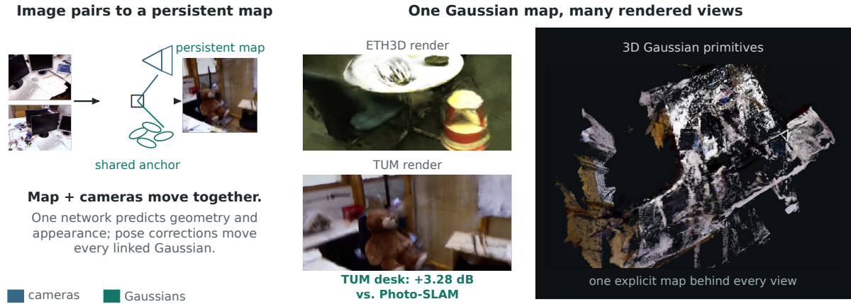
Figure 1.1. A keyframe anchor links the local Gaussian map and the cameras that observe it, so pose corrections move both. The map is shown as individual primitives and rendered from real ETH3D and TUM views; on real desk it is +3.3 dB over Photo-SLAM.
