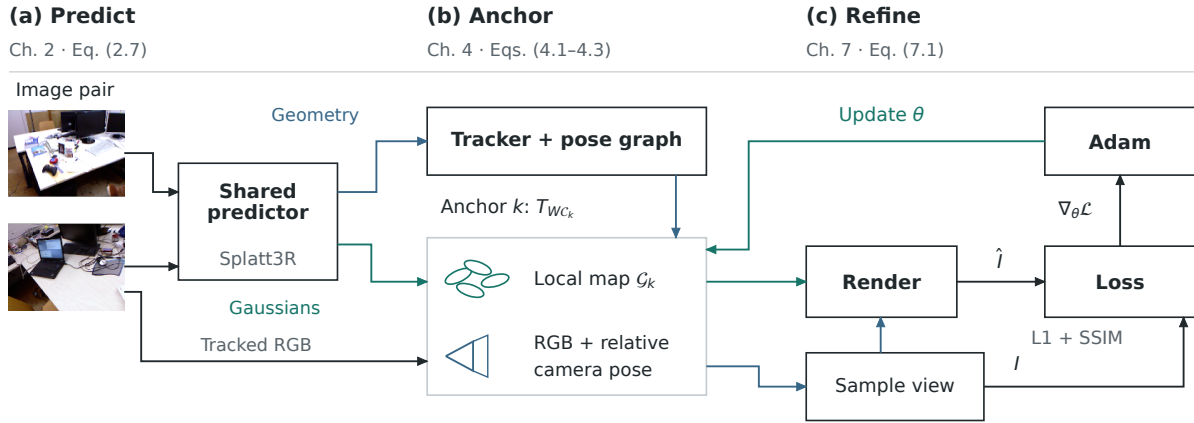
Figure 4.1. Method navigation. Real input frames enter a shared predictor. Geometry feeds tracking, while local Gaussians attach to keyframe anchors. The same anchors carry supervision cameras. A separate process samples observations, renders the map, and updates its appearance. Chapter and equation labels point to the detailed derivation.
