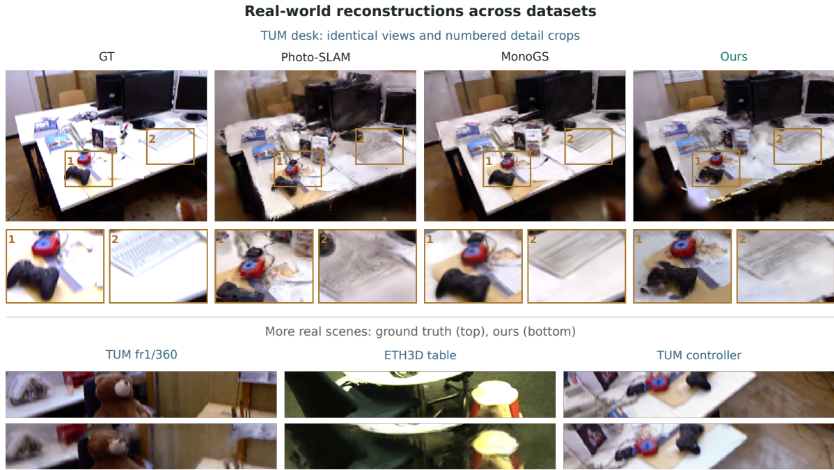
Figure 9.3. Top: TUM desk compared with ground truth, Photo-SLAM, and MonoGS at a common camera. Numbered insets (1: game controllers; 2: keyboard) zoom the same two thin-structure regions across every method. Bottom: further TUM and ETH3D sequences with ground truth above each rendering. Thin structures retain the most blur and geometric distortion.
