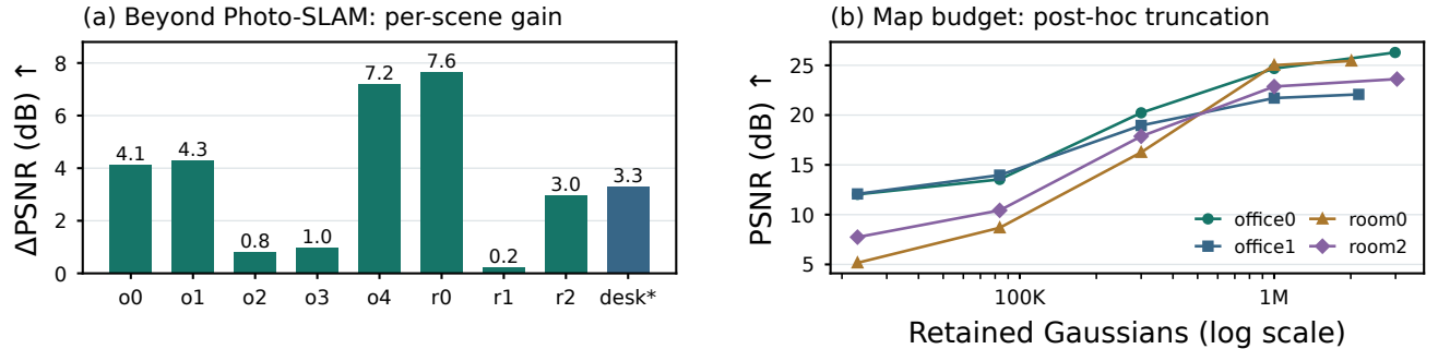
Fig. 5. Beyond Photo-SLAM. (a) Per-scene PSNR improvement of our full-SH map over Photo-SLAM. Teal bars are Replica scenes (synthetic); the blue bar is real TUM desk, where the gain is +3.3 dB. Gains are largest in office4 and room0 and smallest in room1, so the improvement is scene dependent. (b) Post-hoc truncation keeps the highest-opacity primitives of four maps without re-optimisation; quality falls off below about one million Gaussians, with the final marker denoting each full map.
