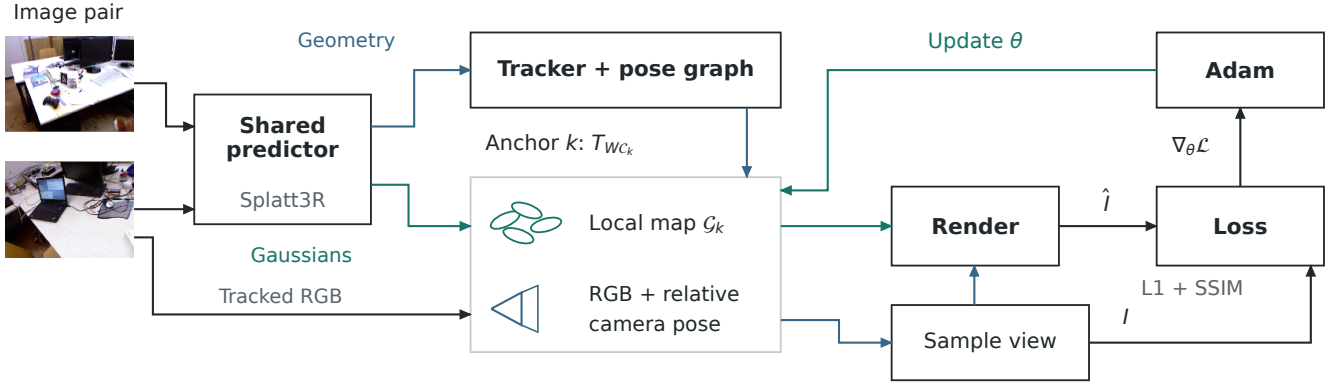
Fig. 2. Predict, anchor, refine. Real TUM frames enter a shared predictor. Its geometric outputs support tracking; its Gaussian outputs form local maps. A keyframe anchor carries each local map and its supervision cameras, so both follow pose corrections. The refiner samples tracked images, renders the assembled map, and updates Gaussian appearance. Section and equation references locate each step.
