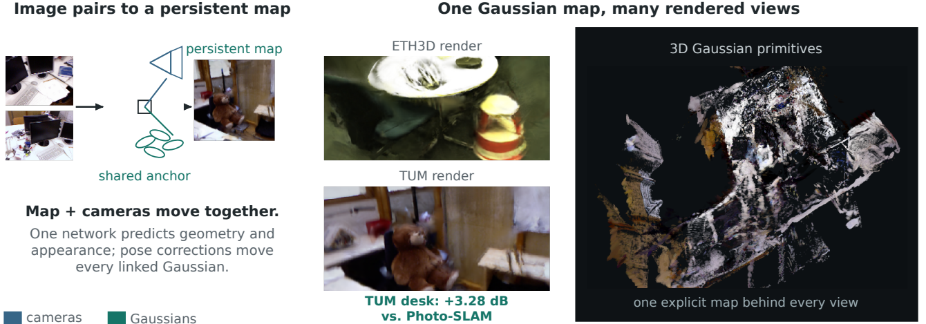
Fig. 1. Image pairs become a persistent map. Left: two images pass one shared predictor; a keyframe anchor links the local Gaussian map and the cameras that observe it, so a pose correction moves both together. Right: the map drawn as individual Gaussian primitives and renders from held-out views on real ETH3D and TUM. On real TUM desk the refined map is +3.28 dB over Photo-SLAM.
