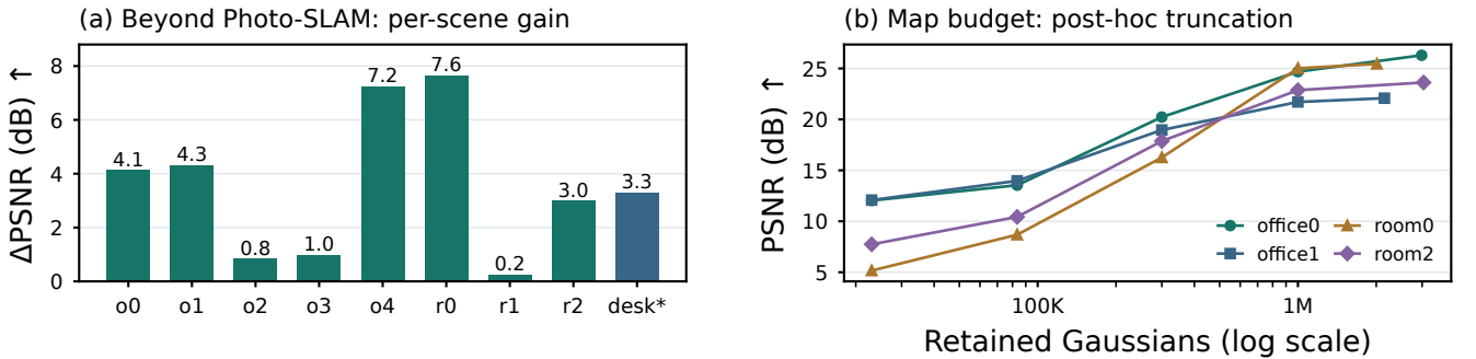
Fig. 5. Beyond Photo-SLAM. (a) Per-scene PSNR improvement of our full-SH map over Photo-SLAM. Teal bars are Replica scenes (synthetic); the blue bar is real TUM desk, where the gain is +3.3dB. Gains are largest in office4 and room0 and smallest in room1, so the improvement is scene dependent. (b) Post-hoc truncation keeps the highest-opacity primitives of four maps without re-optimisation; quality falls off below about one million Gaussians, with the final marker denoting each full map.
