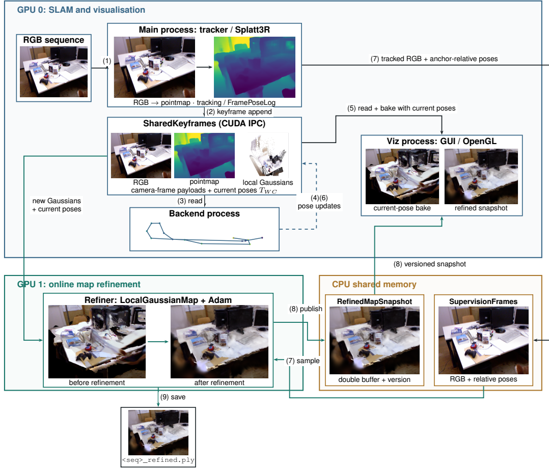
Fig. 3. System overview. Tracking, pose-graph optimisation, and visualisation run on GPU 0. The optional map refiner runs on GPU 1. SharedKeyframes uses CUDA IPC; supervision frames and versioned refined-map snapshots use CPU shared memory. Numbered arrows show RGB, predicted pointmaps, local Gaussians, supervision and refined-map flow; dashed arrows denote pose updates. Thumbnails use real TUM desk predictions and recorded maps. Before/after renders share one camera; the backend inset shows recorded keyframe camera centres.
