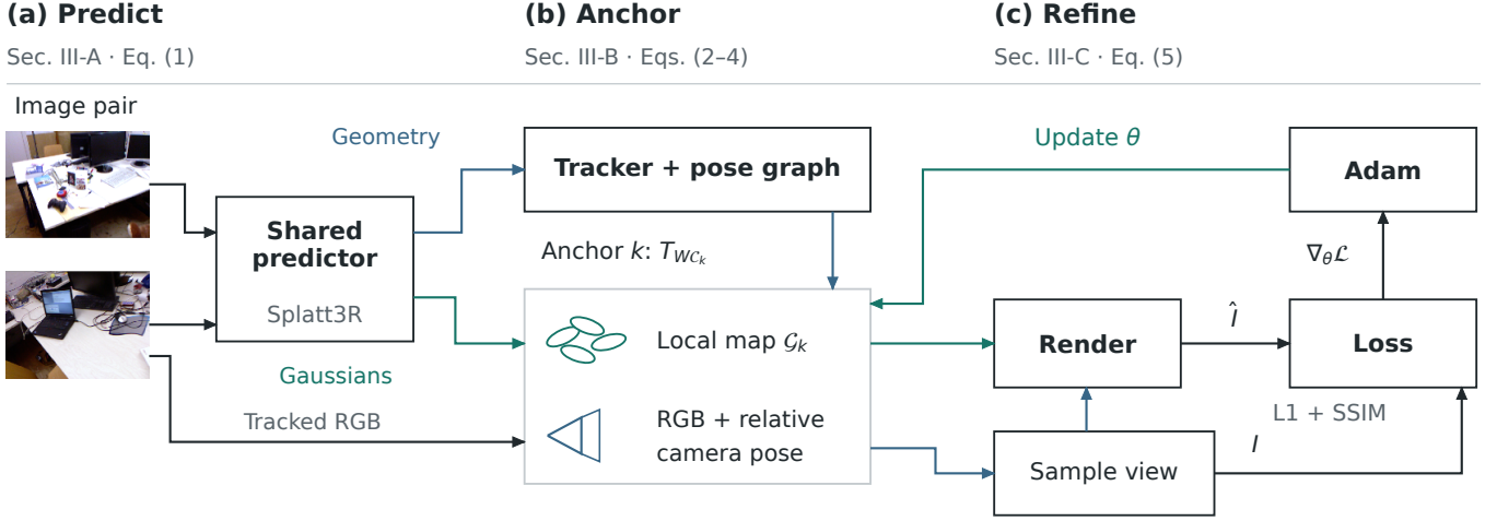
Fig. 2. Predict, anchor, refine. Real TUM frames enter a shared predictor. Its geometric outputs support tracking; its Gaussian outputs form local maps. A keyframe anchor carries each local map and its supervision cameras, so both follow pose corrections. The refiner samples tracked images, renders the assembled map, and updates Gaussian appearance. Section and equation references locate each step.
