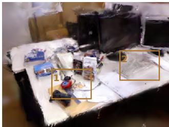
Photo-SLAM
