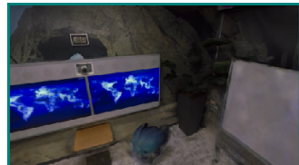
Splatt3R-SLAM
