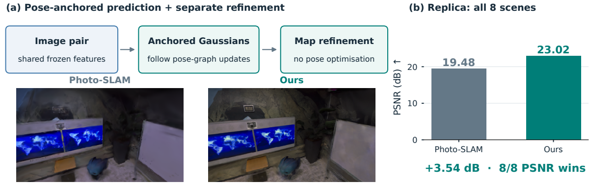
Figure 1.1. Splatt3R-SLAM predicts local Gaussian maps, carries them with keyframe anchors, and refines their appearance. The image is a middle-ranked Replica office0 comparison. The chart reports all eight Replica scenes with common non-keyframe cameras and full exported SH.
