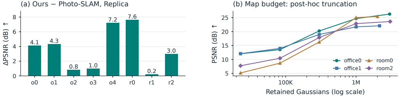
Fig. 4. Quality distribution and map budget. (a) Fresh full-SH scene PSNR differences on Replica; o/r denote office/room. (b) A separate recorded study retaining the highest-opacity primitives in four of our maps, without re-optimisation. The final marker is each full map, containing 2.0–3.0 million Gaussians. The study measures post-hoc removal from maps optimised at full size.
