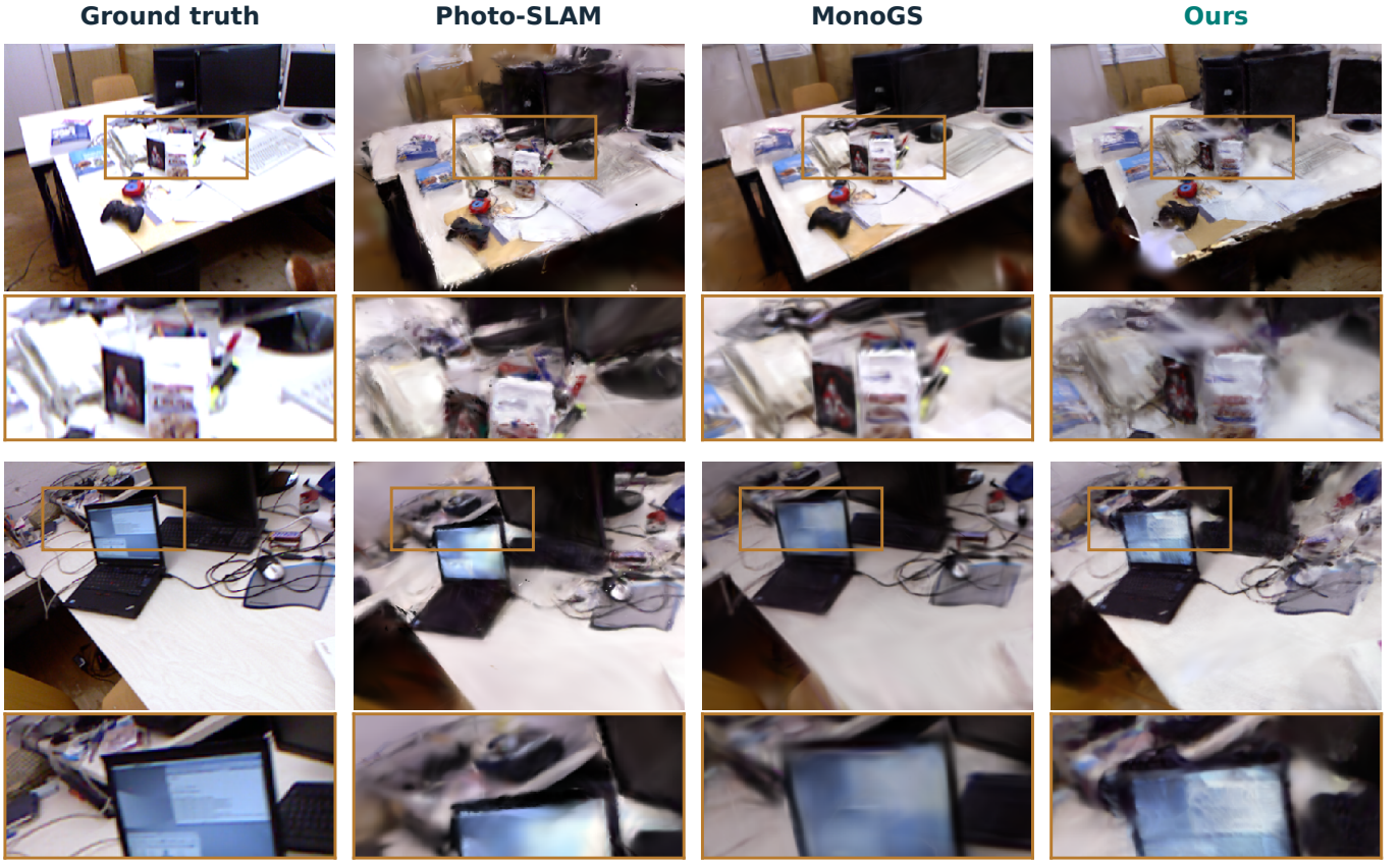
Fig. 3. Related-work comparison on TUM desk. Each method occupies one column; each view is followed by an identically located crop (orange box). The two views are the middle ranks of the per-frame Ours-minus-MonoGS PSNR difference among the 100 common evaluation frames. All columns use the same target camera and image scale. The close quantitative comparison is reflected in remaining blur and geometric distortion in both MonoGS and our renderings.
