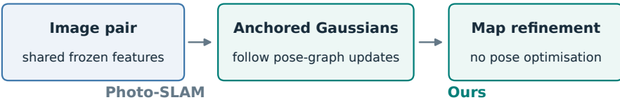
(a) Pose-anchored prediction + separate refinement
