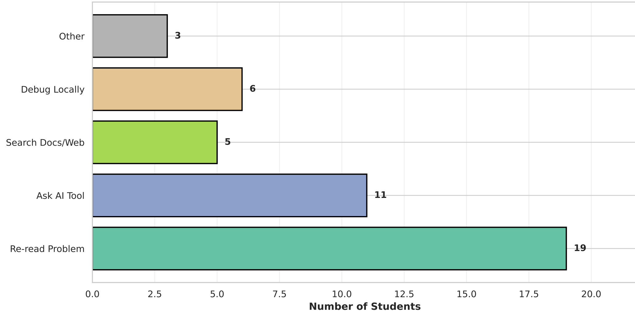
Problem-Solving Strategy: "When Stuck, I Do First..." (n=44: FR=44, EN=6)
