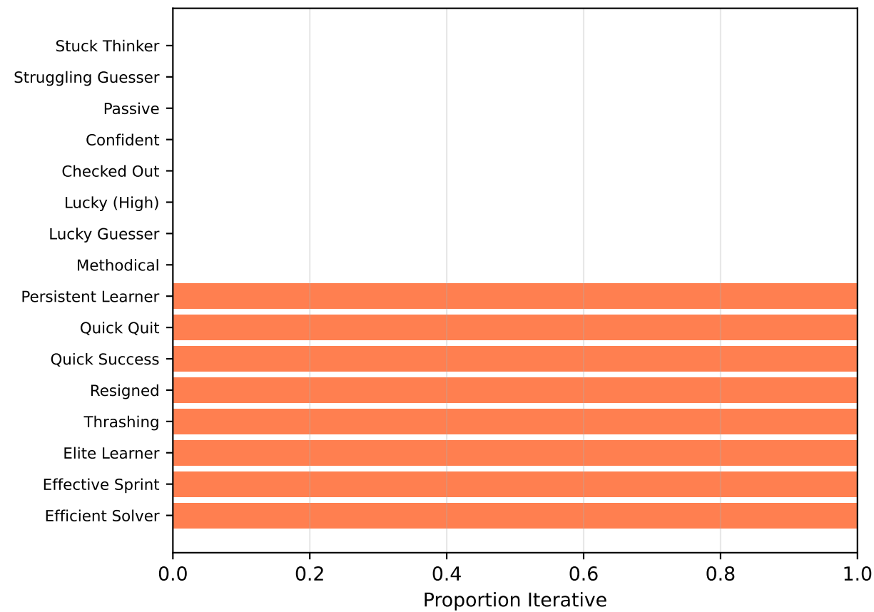
Iterative Dimension
