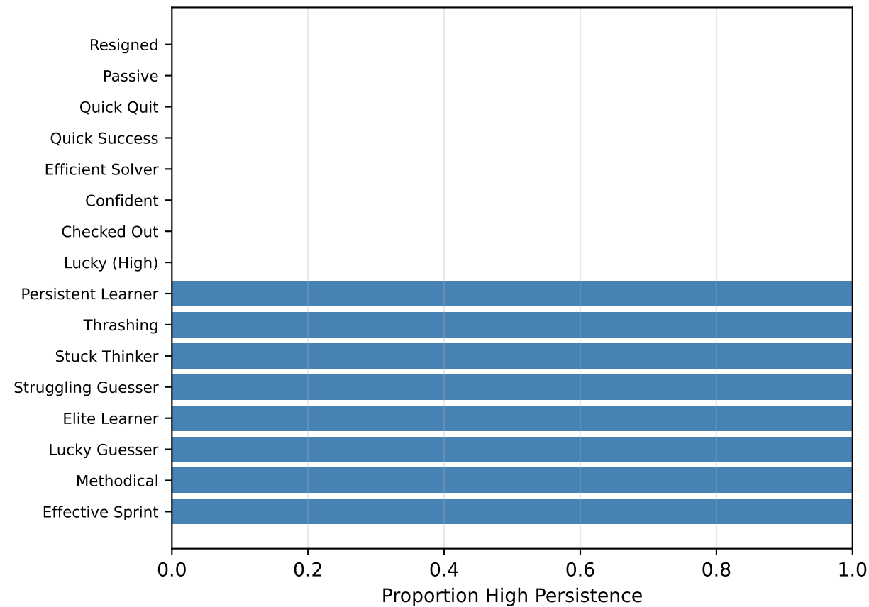
Iterative Dimension
