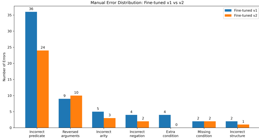
Figure 3: Distribution of manually identified errors for Fine-Tuned v1 and Fine-Tuned v2.
